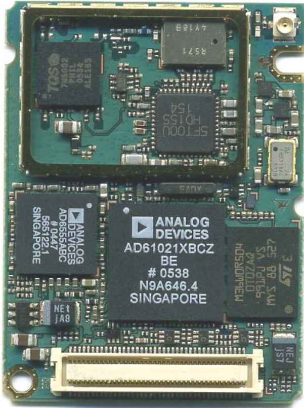
MC75: component side shielding opened
