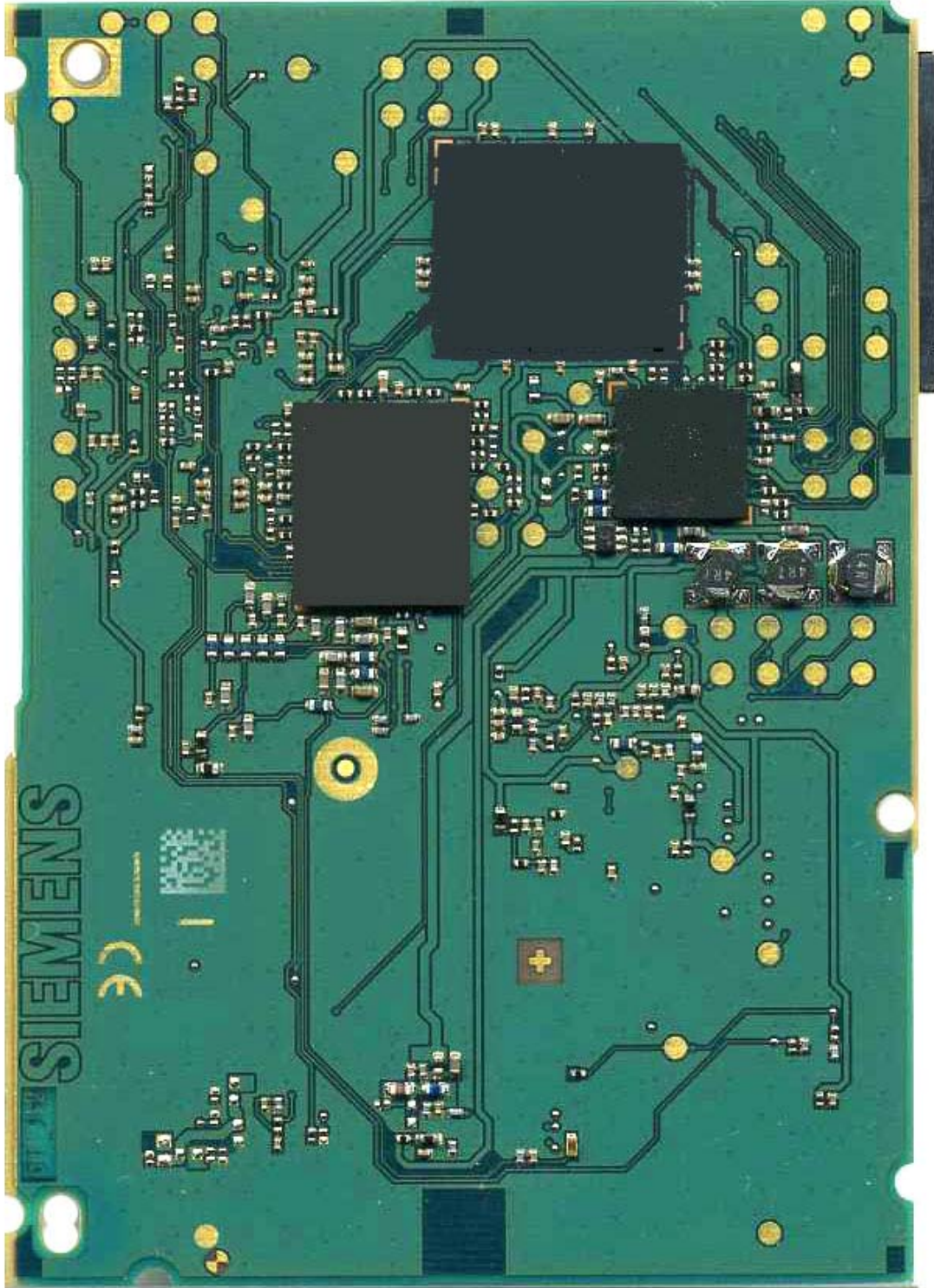
Photo 2: EUT (bottom side of module) picture provided by manufacturer and may not show the tested sample.
