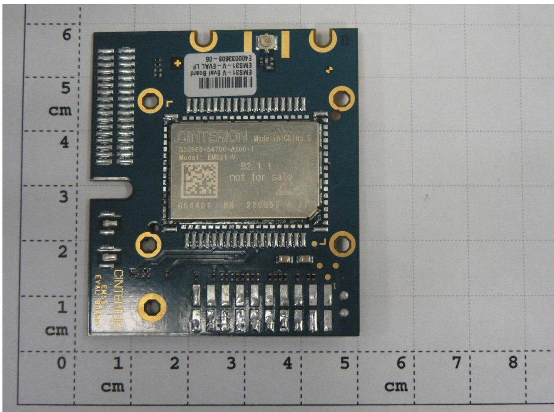
Photograph 3: EUT B - Front side view
