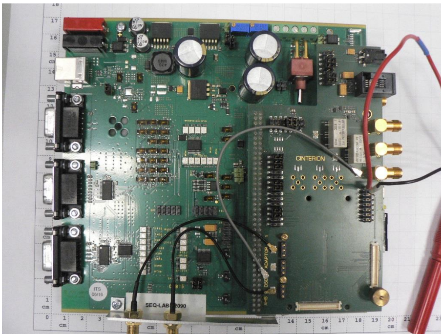
Photograph 5: AE2 front side + AE 3 front side + AE 4(gray cable)
