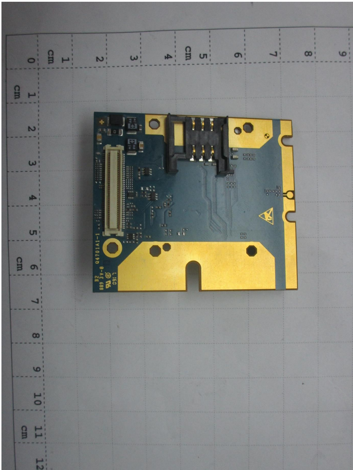
EUT under side
