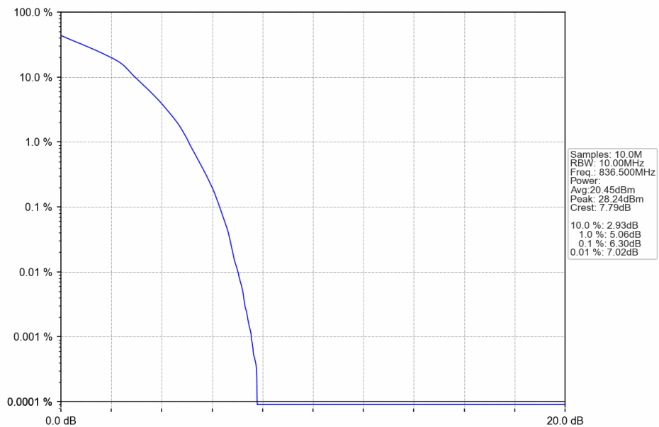
Band5 10MHz 16QAM MCH 836.5MHz RB 27 0 NTNV
