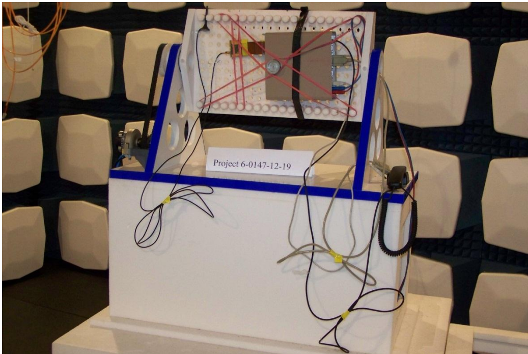
Radiated field strength measurements in the FAR (Fully-Semi-Anechoic-Chamber)
