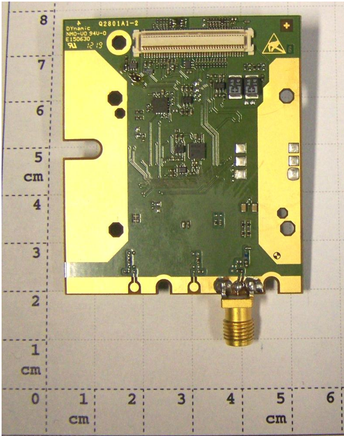
EUT A on Test Adapter (AE 7) – bottom side view
