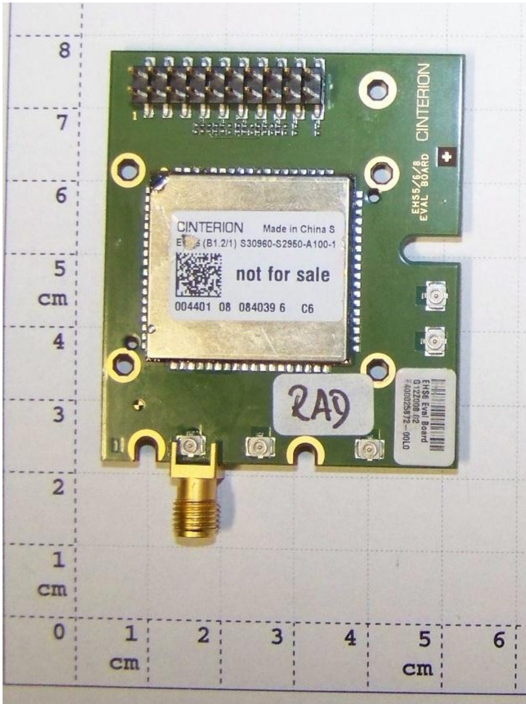
EUT A on Test Adapter (AE 7) – top side view
