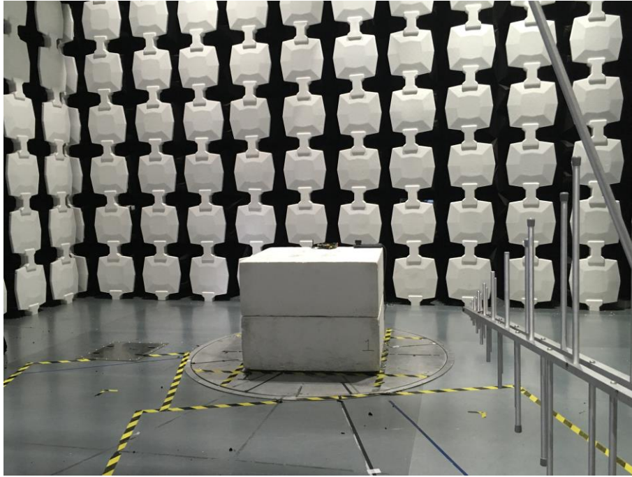
Test Mode: Mode 1 Description: Backview of Radiated Emission Test Setup
