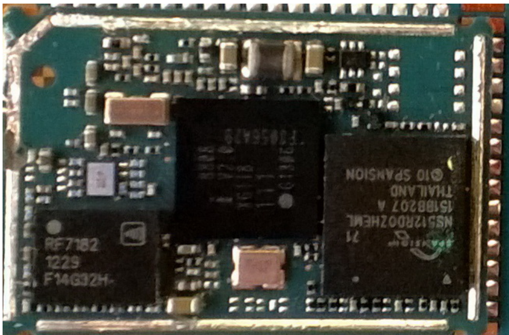
Module Disassembly
