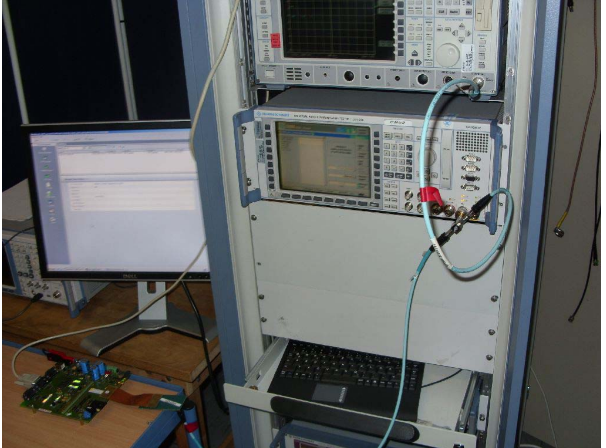
setup for conducted testing
