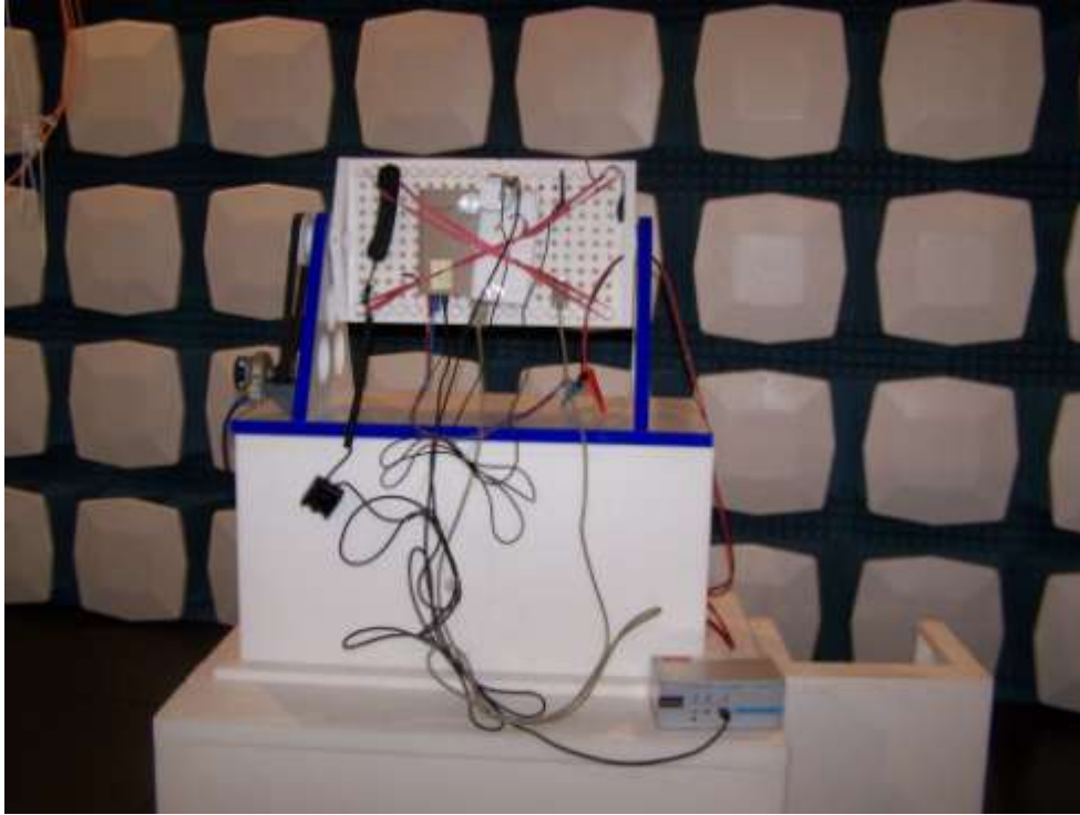
Photographs: Radiated measurements set-up
