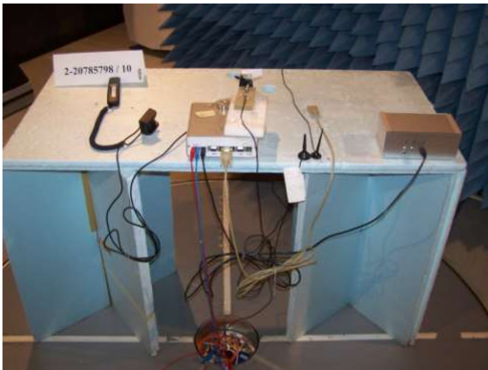
Photographs: Radiated measurement set-up
