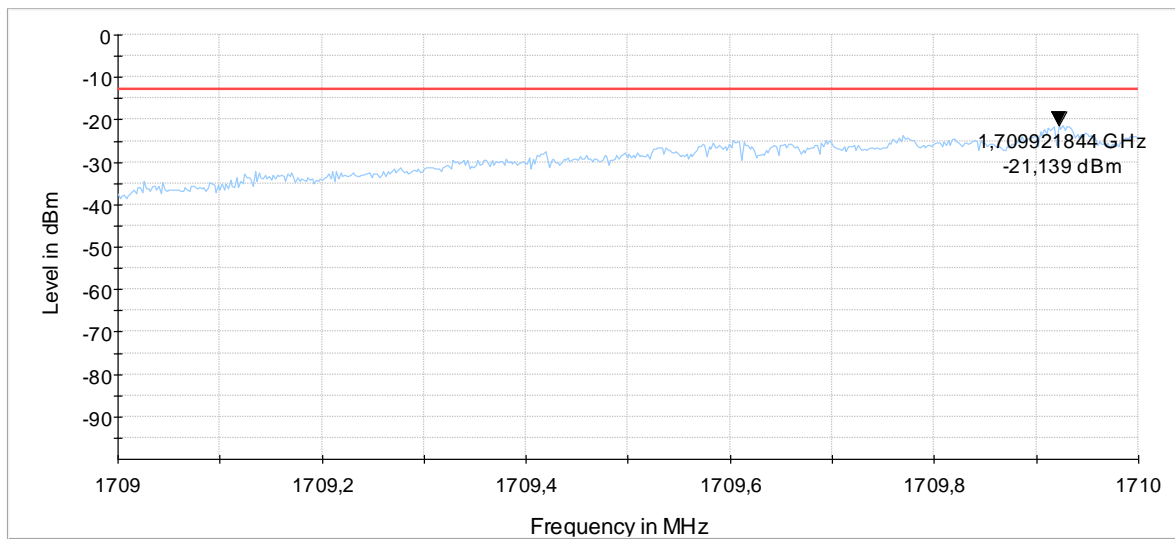
Diagram 9.519b, Channel 19957, 16-QAM, 6RBs
