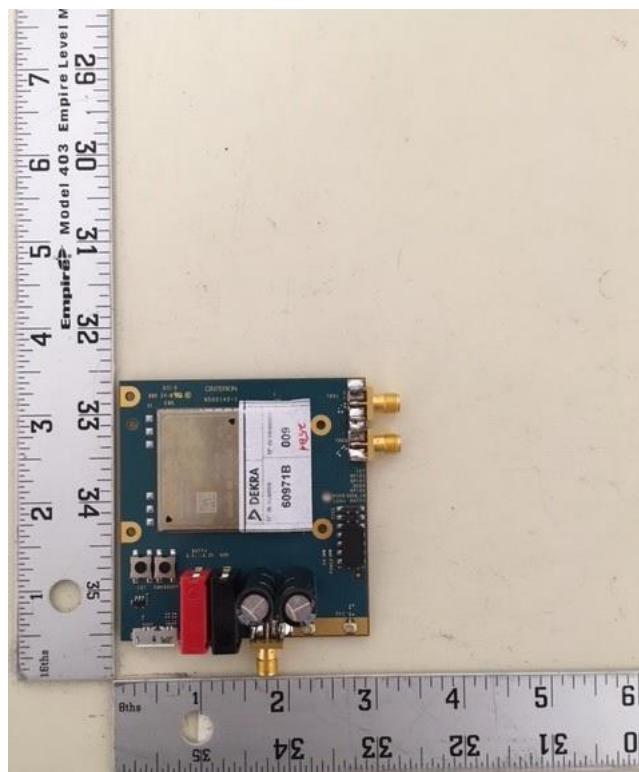
Figure B2. DUT Module only top view
