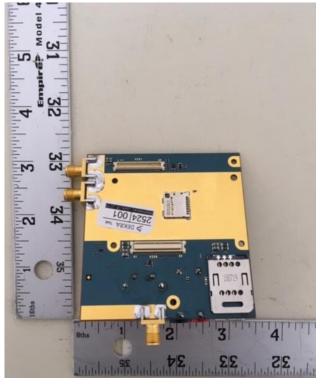
Figure B3. DUT Module only rear view
