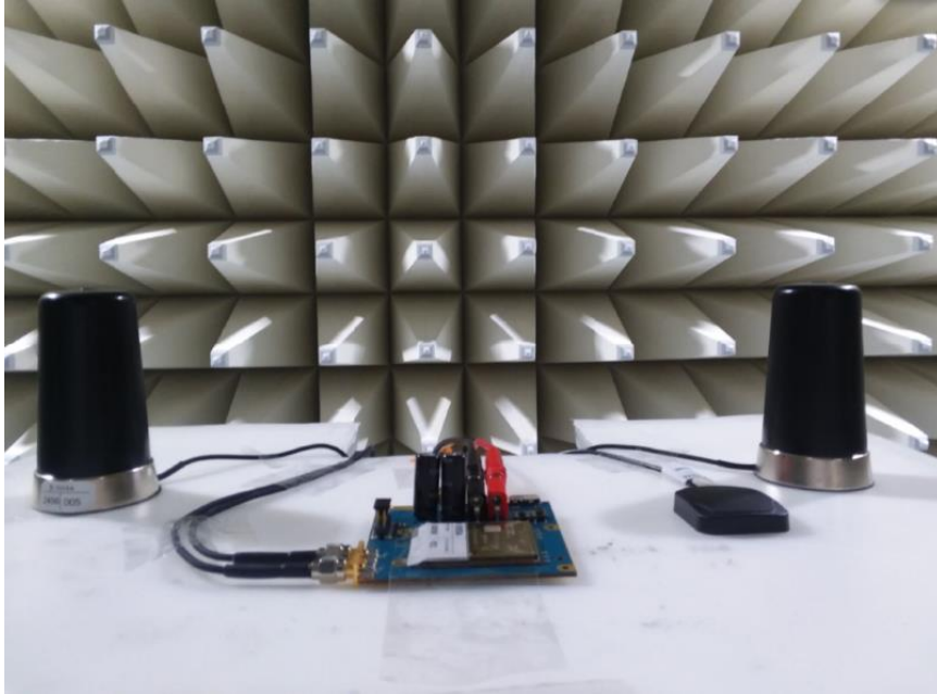
Figure B5. Radiated emission Set up
