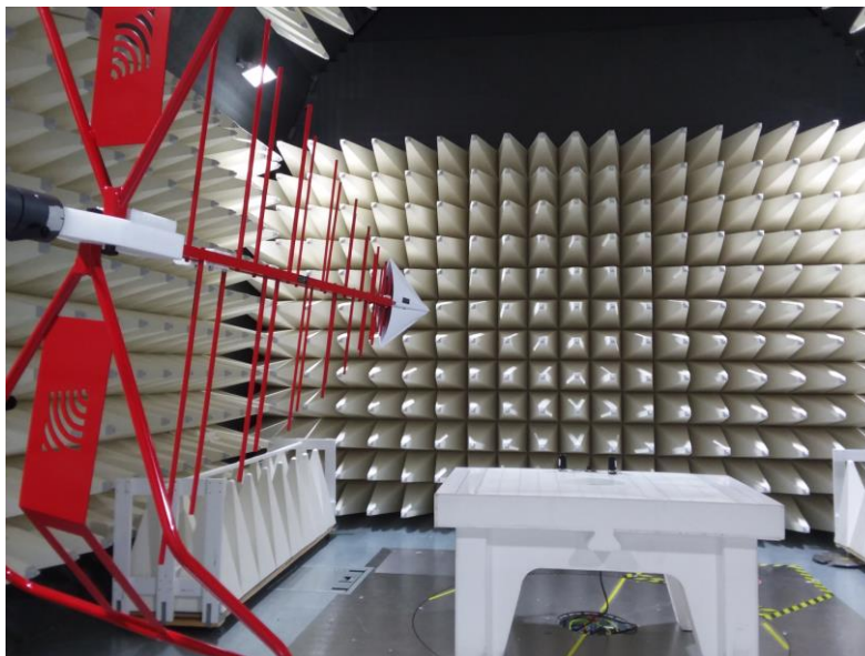
Figure B4. Low range Radiated emission Set up Biconical log antenna
