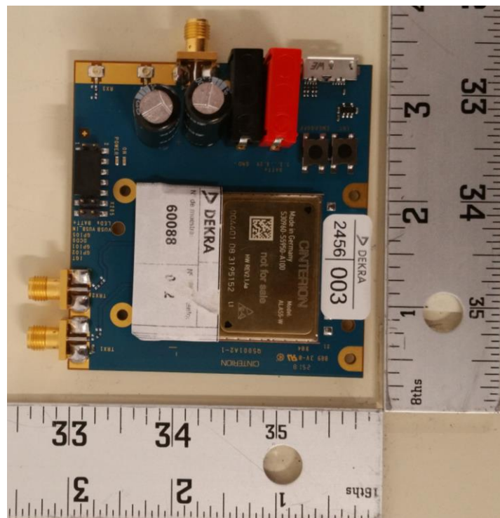
Figure B2. DUT Module only top view
