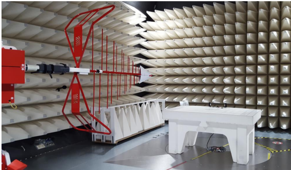
Figure B4. Radiated Set up 1
