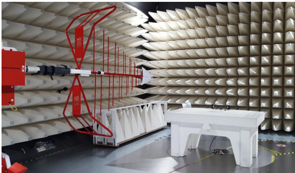
Figure B4. Radiated emission Set up 1
