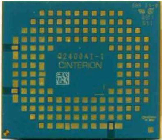
AHS3-W Bottom side
