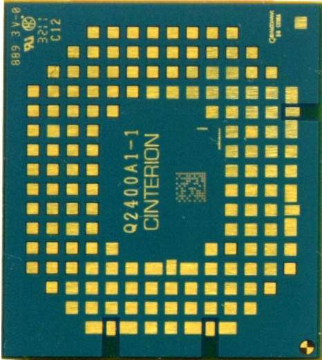
AHS3-W Bottom Side
