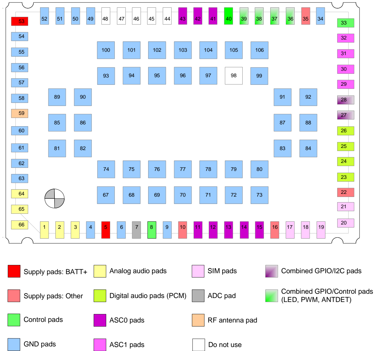
Figure 1: Numbering plan for connecting pads (bottom view)
