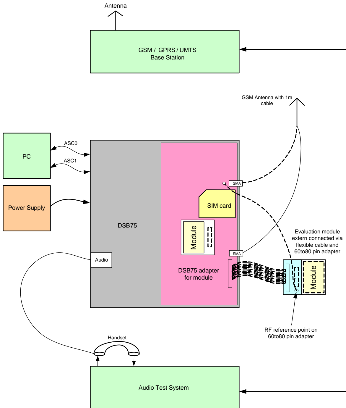
Figure 3: Reference equipment for Type Approval
