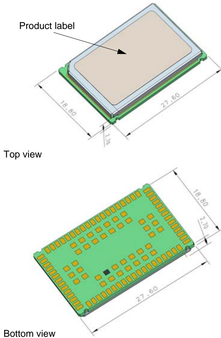
Figure 2: AGS2-W– top and bottom view
