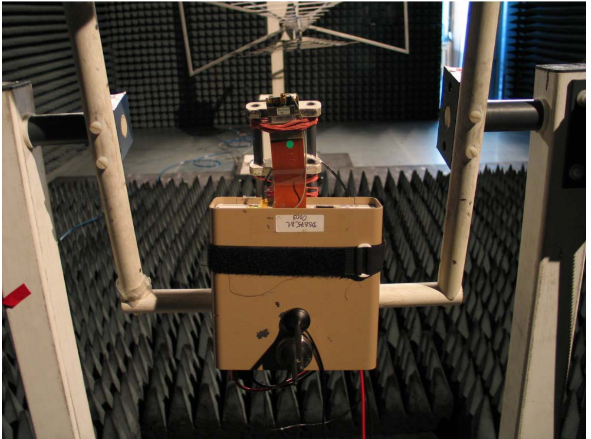
setup for radiated testing
