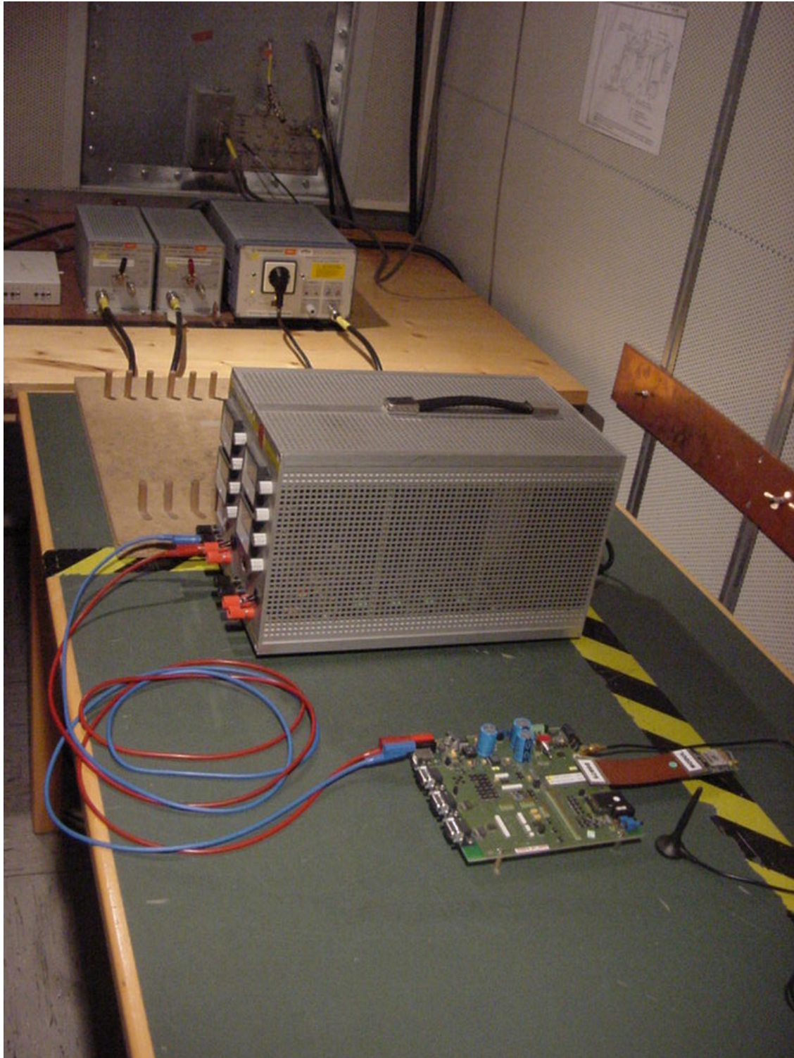
Photo 3 (Conducted Emissions):
