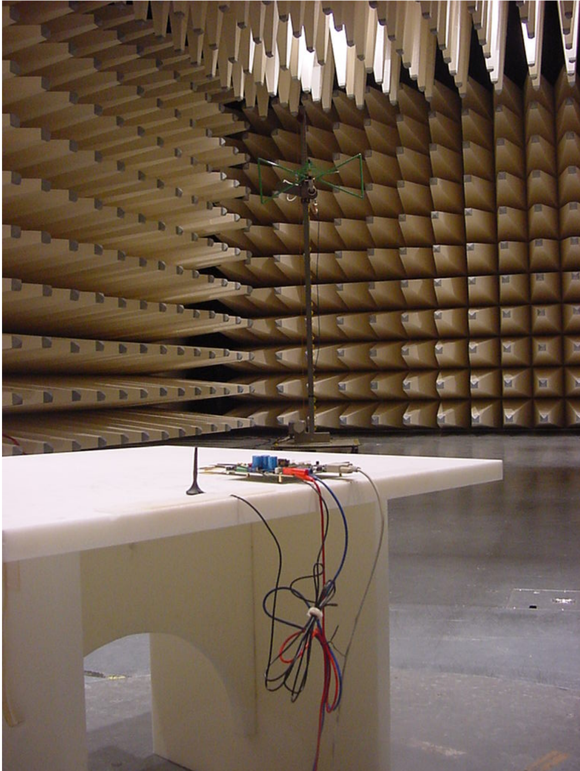
Photo 1 (Radiated Emissions):
