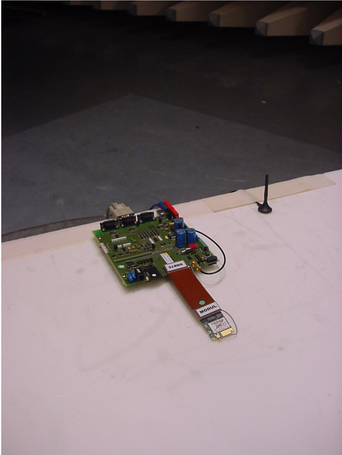
Photo 2 (Radiated Emissions):
