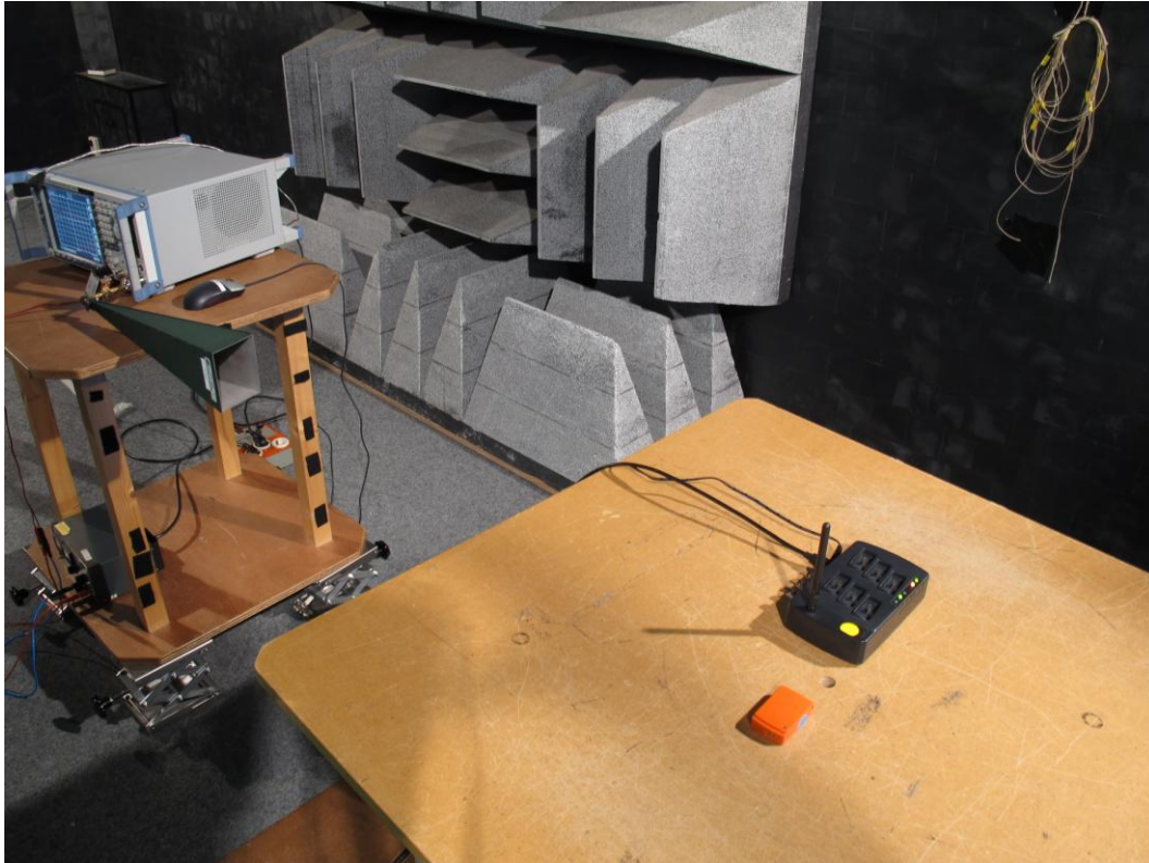
Photograph 3: - MTw sensor, test setup radiated emissions (18 - 26 GHz)
