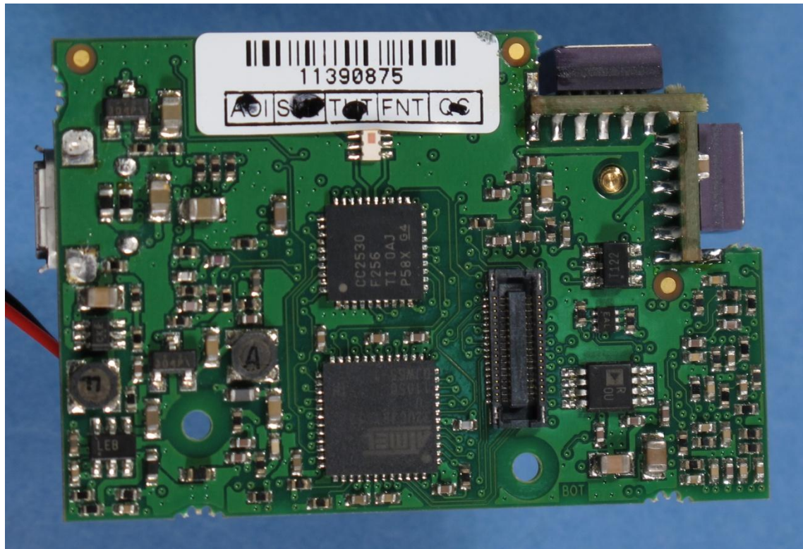
Photograph 4: - MTw sensor, bottom view of PCB
