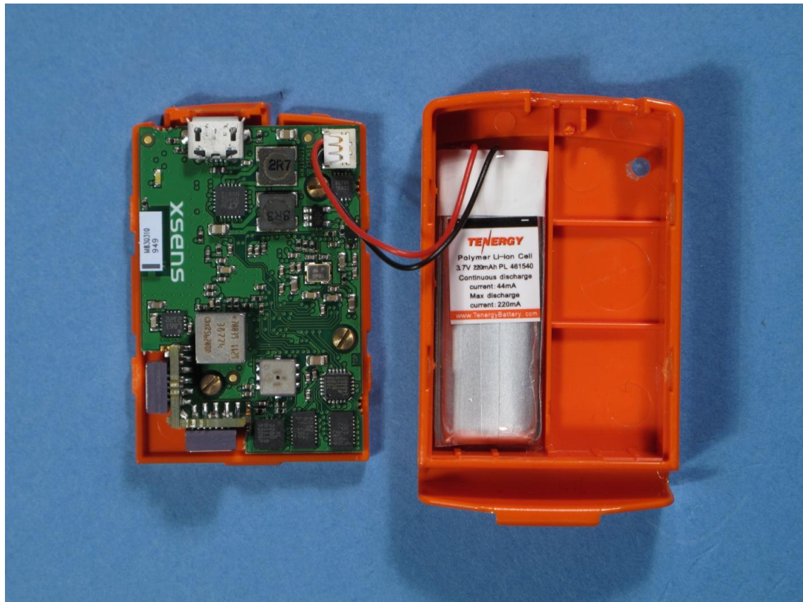
Photograph 1: - MTw sensor, internal view
