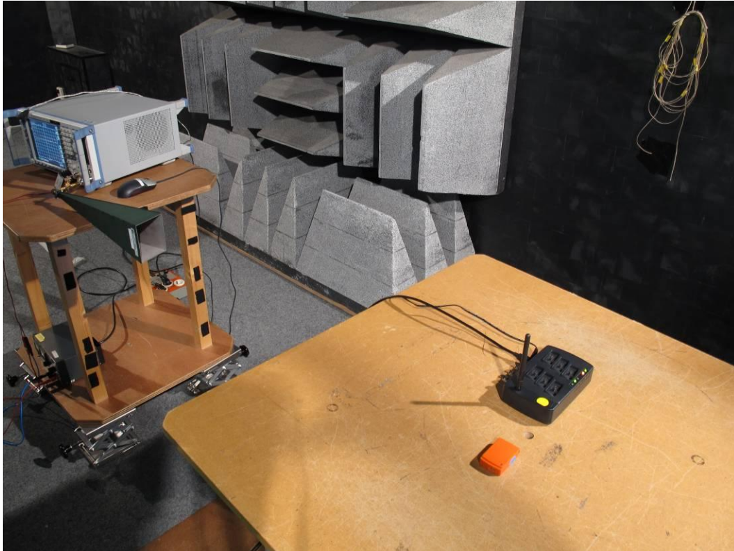
Photograph 3: - MTw , test setup radiated emissions (18 - 26 GHz)
