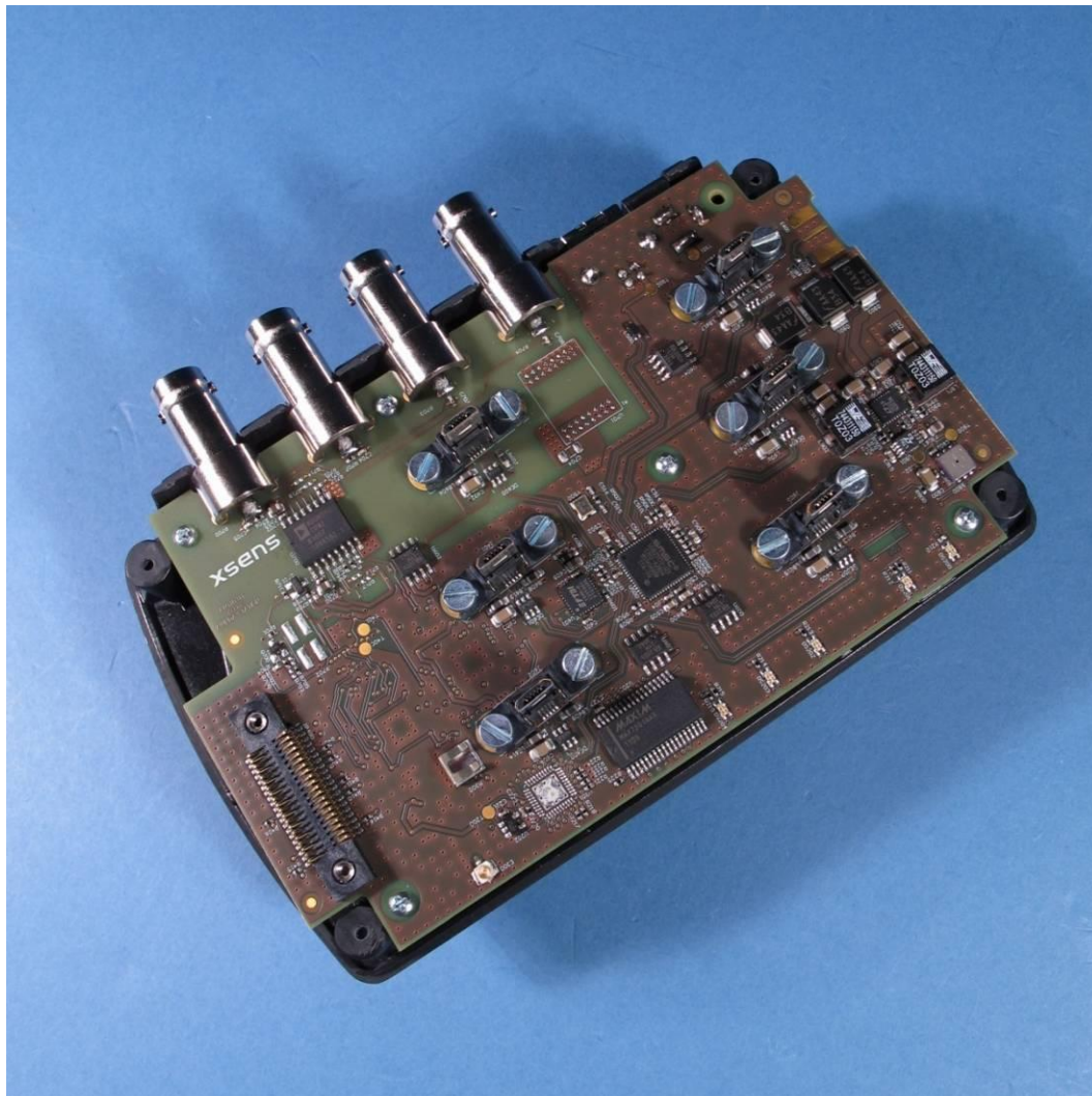
Photograph 2: - AW-A Wireless base station, battery view
