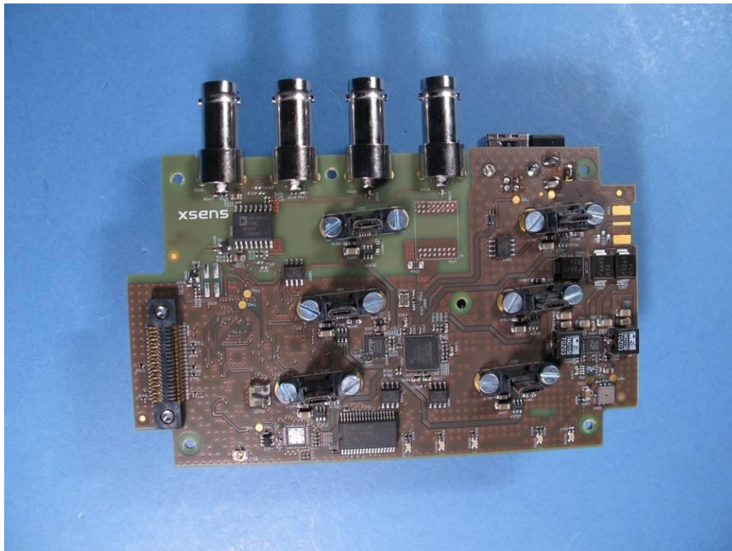
Photograph 3: - AW-A Wireless base station, top view of PCB
