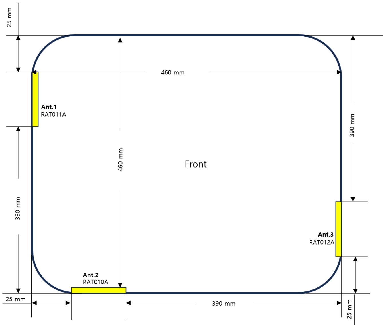
Figure E-1 Antenna Location (Front Side View)
