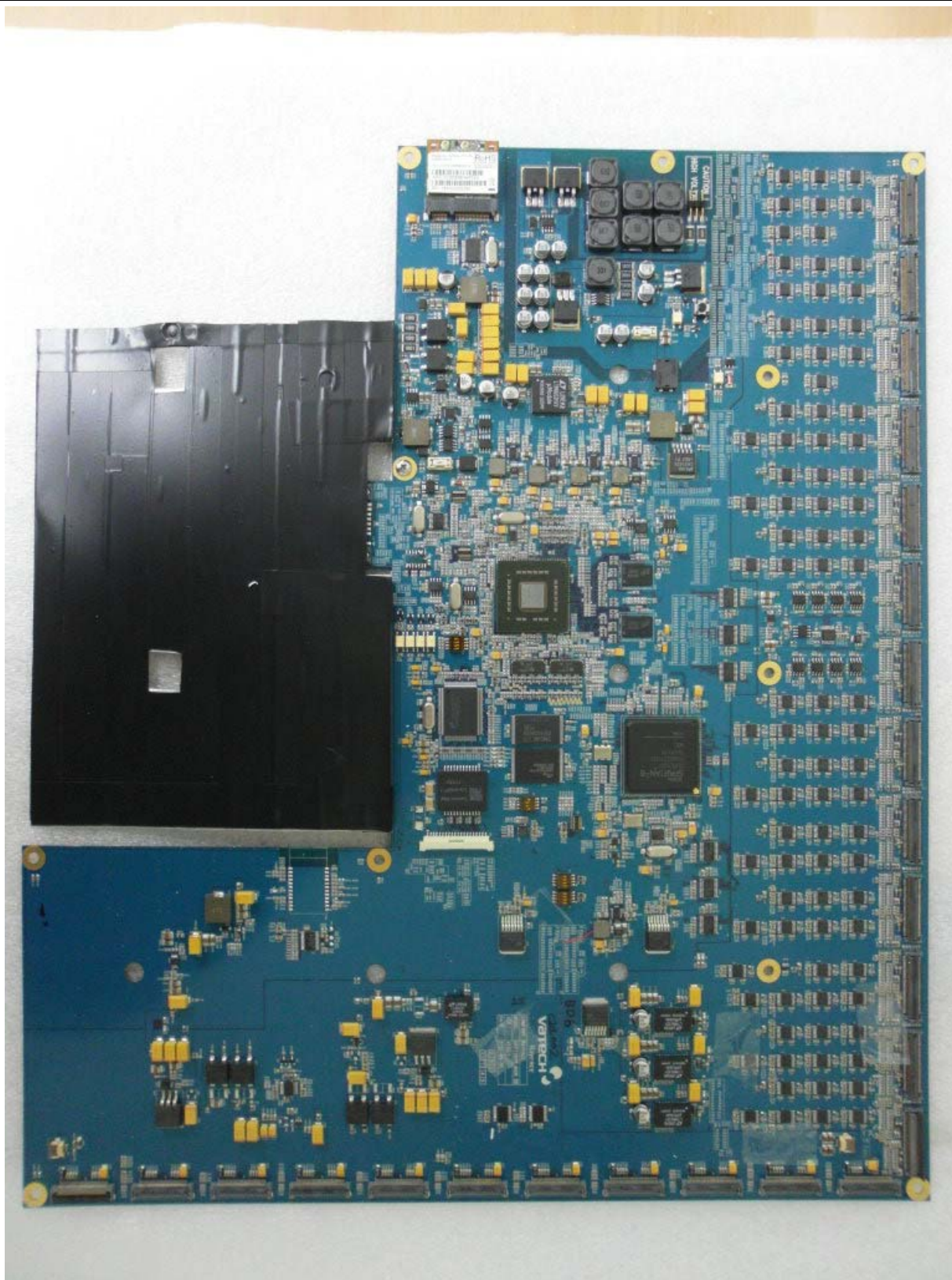
Main board
