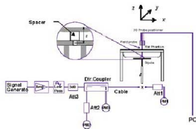
Figure 9.1 Dipole Verification Test Setup Diagram & Photo
