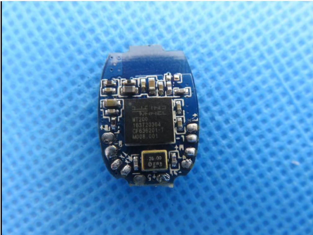
INTERNAL VIEW OF EUT-7 (Right)
