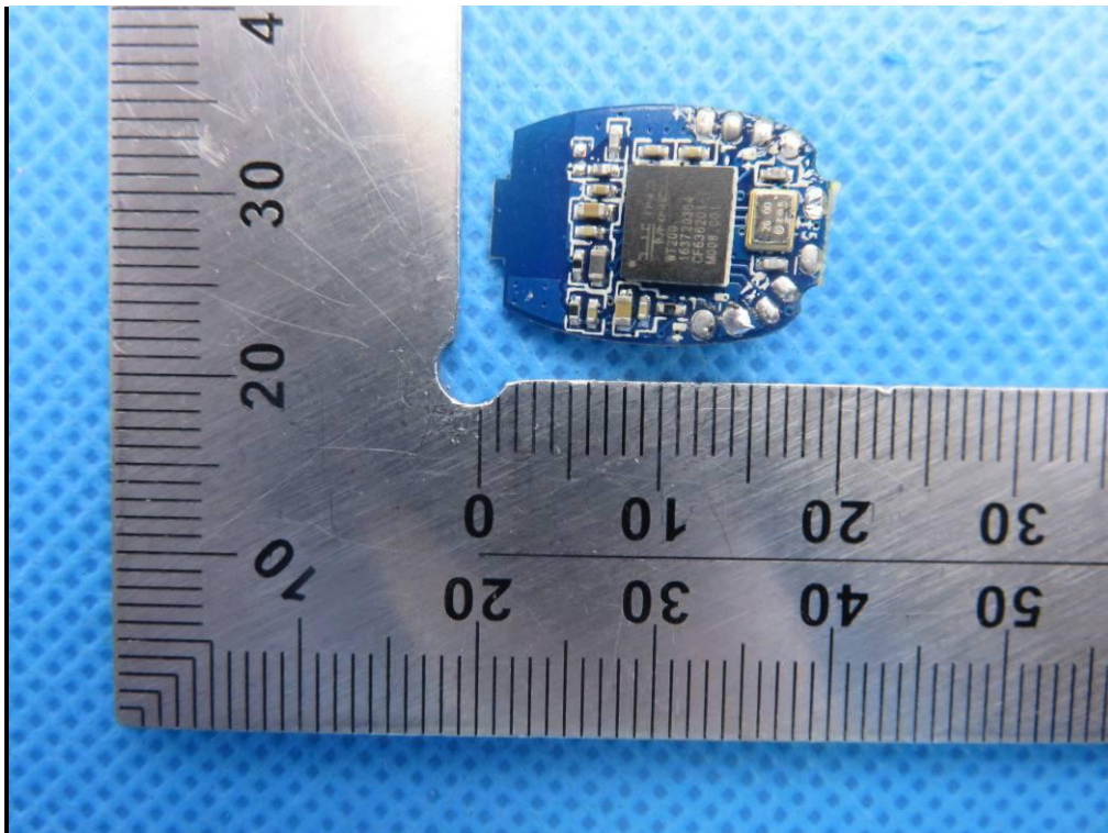
INTERNAL VIEW OF EUT-6 (Right)
