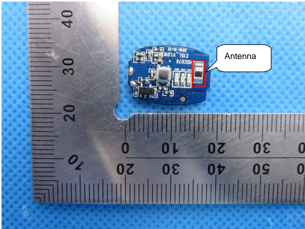
INTERNAL VIEW OF EUT-6 (Left)
