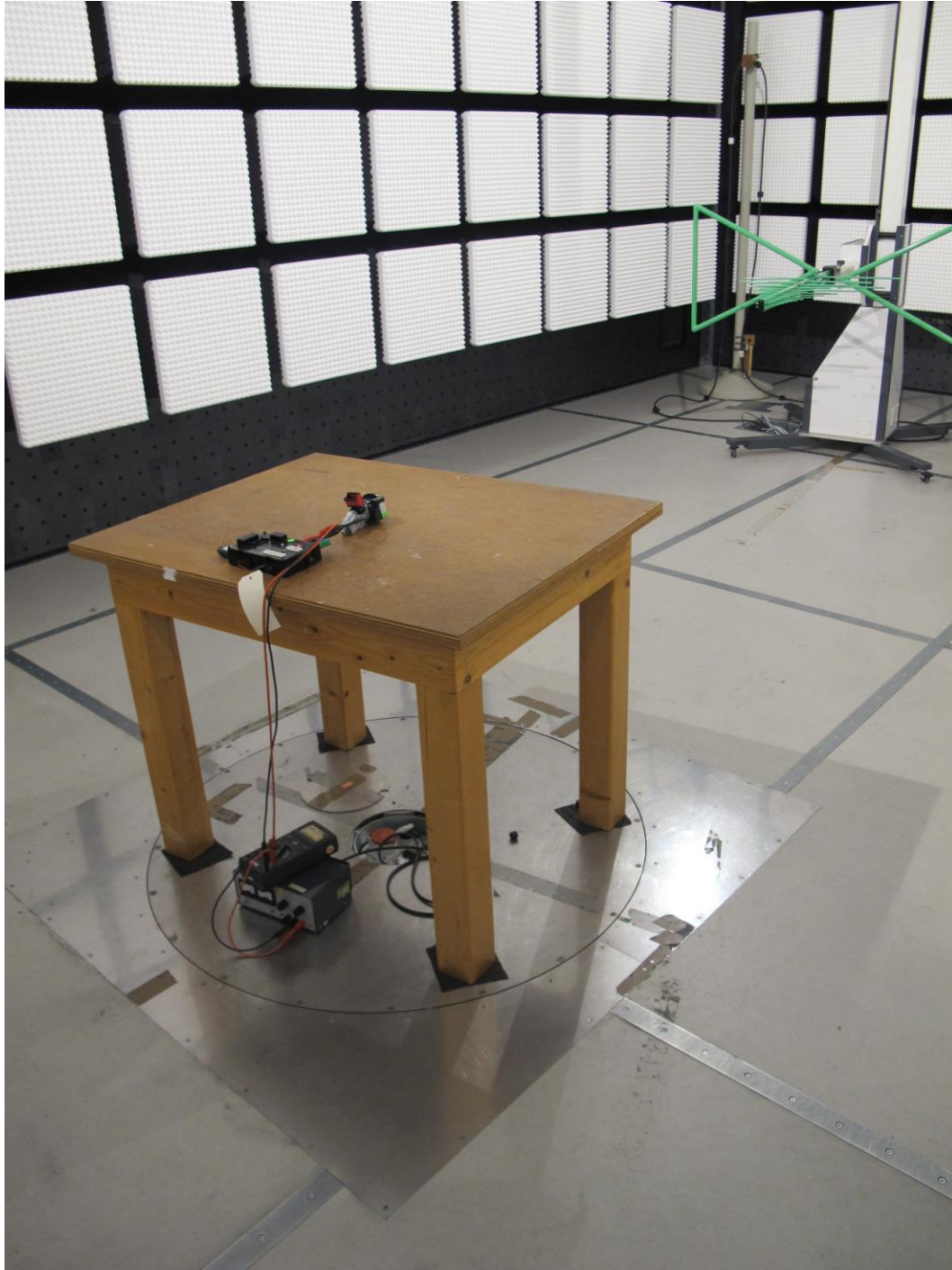
Photograph 2: Test setup radiated emissions 30-1000 MHz)
