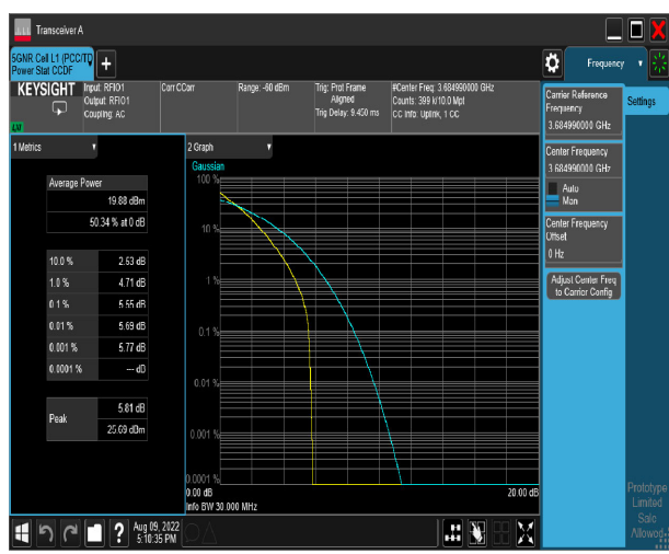
30MHz_QPSK_CH645666
