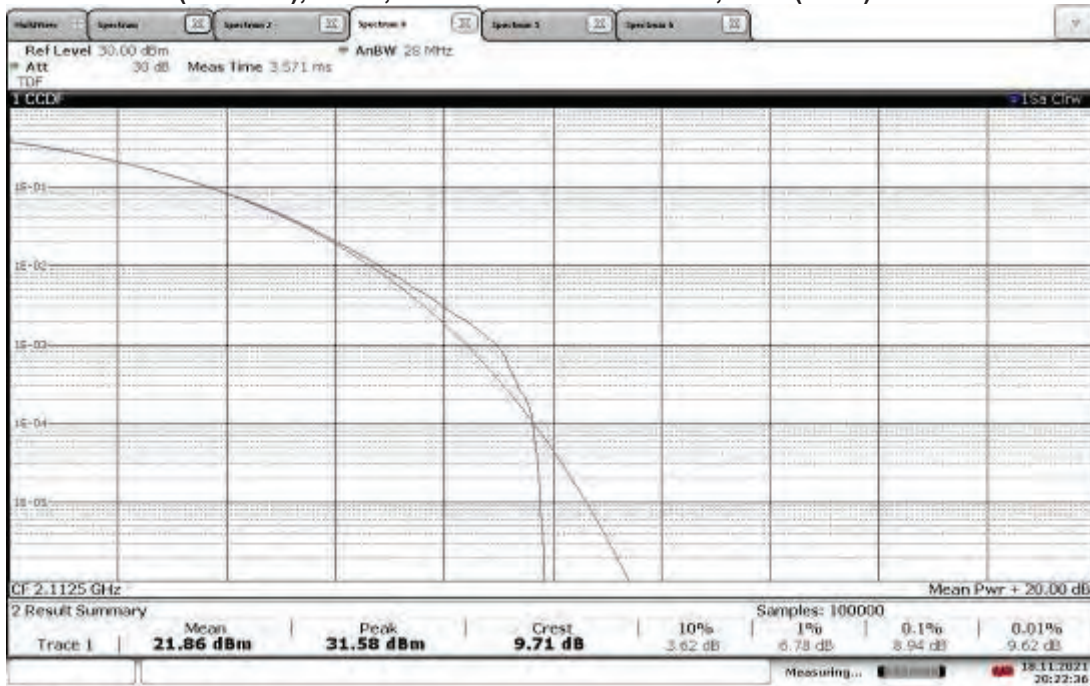
TM1.1-QPSK_5 MHz Bandwidth Slot 2(Band 66), ANT0, Low Channel 2112.5 MHz, PAR (0.1%) = 8.94 dB
