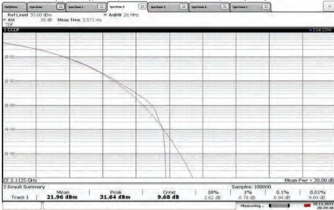
TM1.1-QPSK_5 MHz Bandwidth Slot 2(Band 66), ANT1, Low Channel 2112.5 MHz, PAR (0.1%) = 8.94 dB
