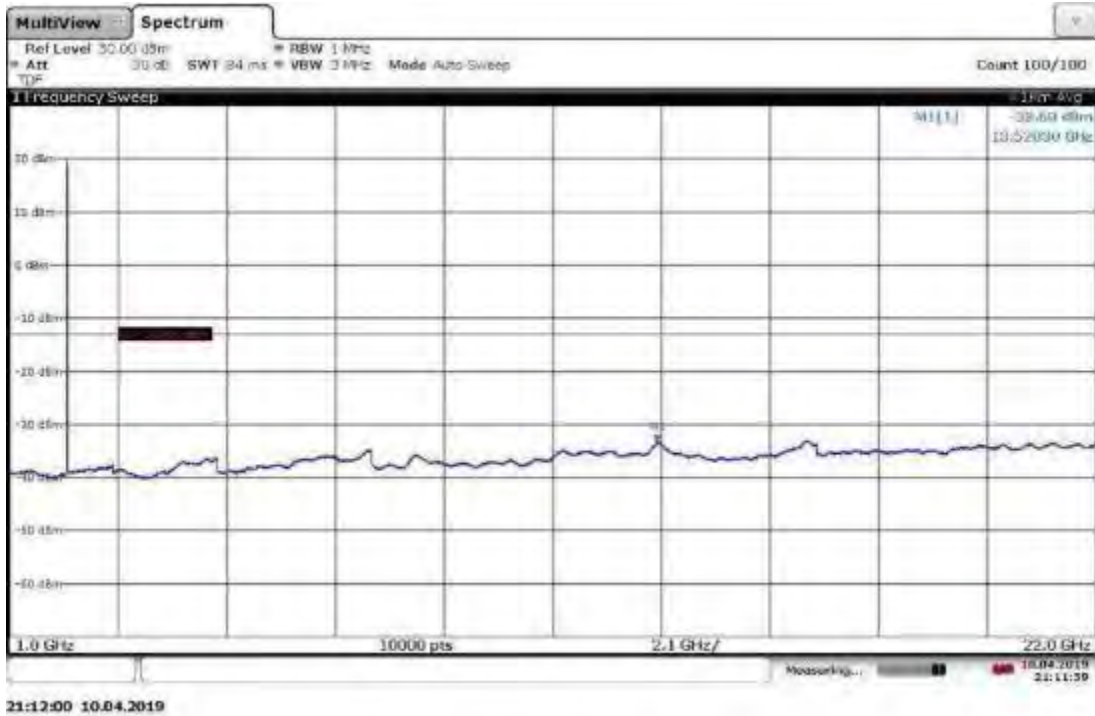
Slot 1 (Band 10), ANT0, Modulation: TM1.1-QPSK, Bandwidth: 5 MHz, Low Channel 1-22GHz
