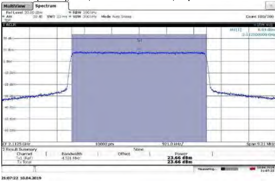
TM1.1-QPSK_5 MHz Bandwidth Slot 1 (Band 10), ANT0, Low Channel 2112.5 MHz, Output Power = 23.66 dBm
