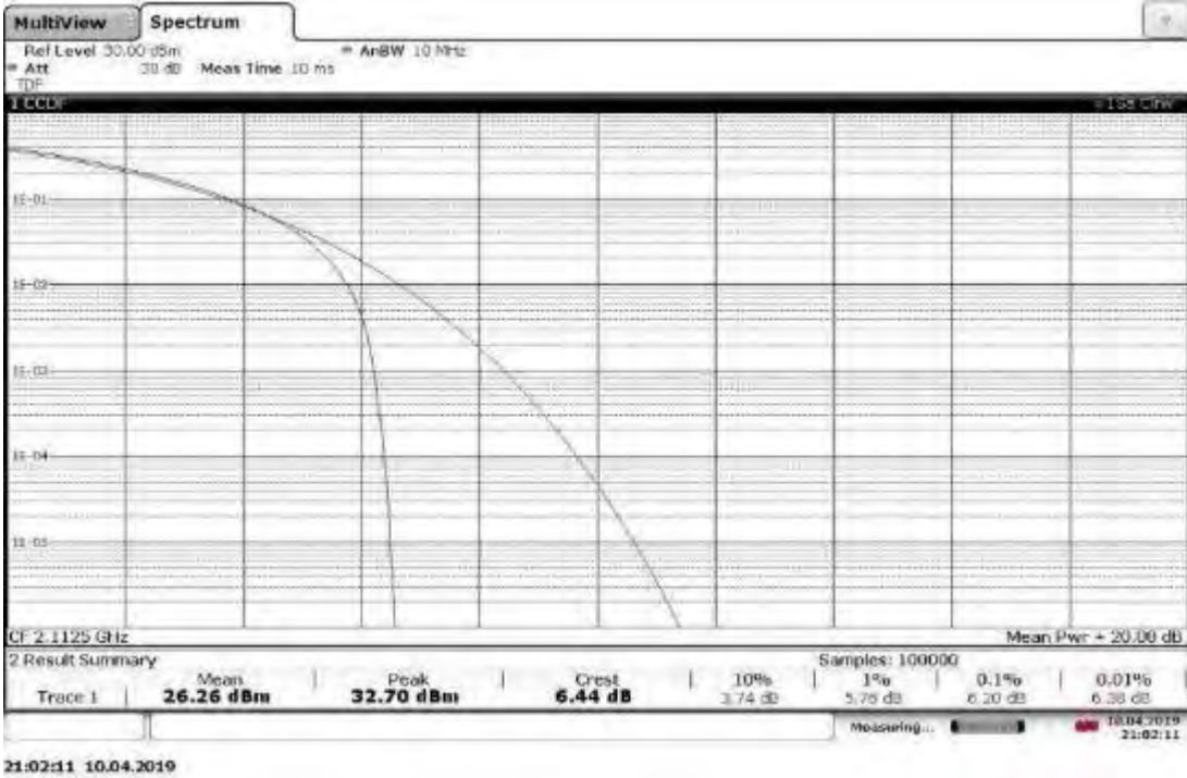
TM1.1-QPSK_5 MHz Bandwidth Slot 1 (Band 10), ANT1, Low Channel 2112.5 MHz, PAPR = 6.44 dB
