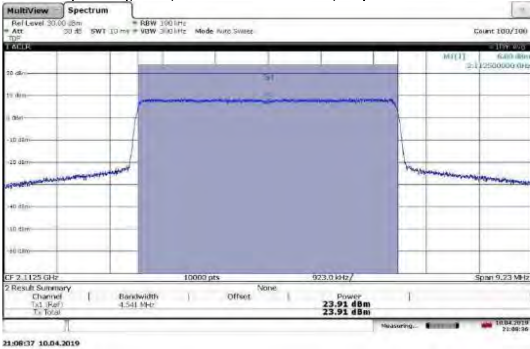
TM1.1-QPSK_5 MHz Bandwidth Slot 1 (Band 10), ANT1, Low Channel 2112.5 MHz, Output Power = 23.91 dBm
