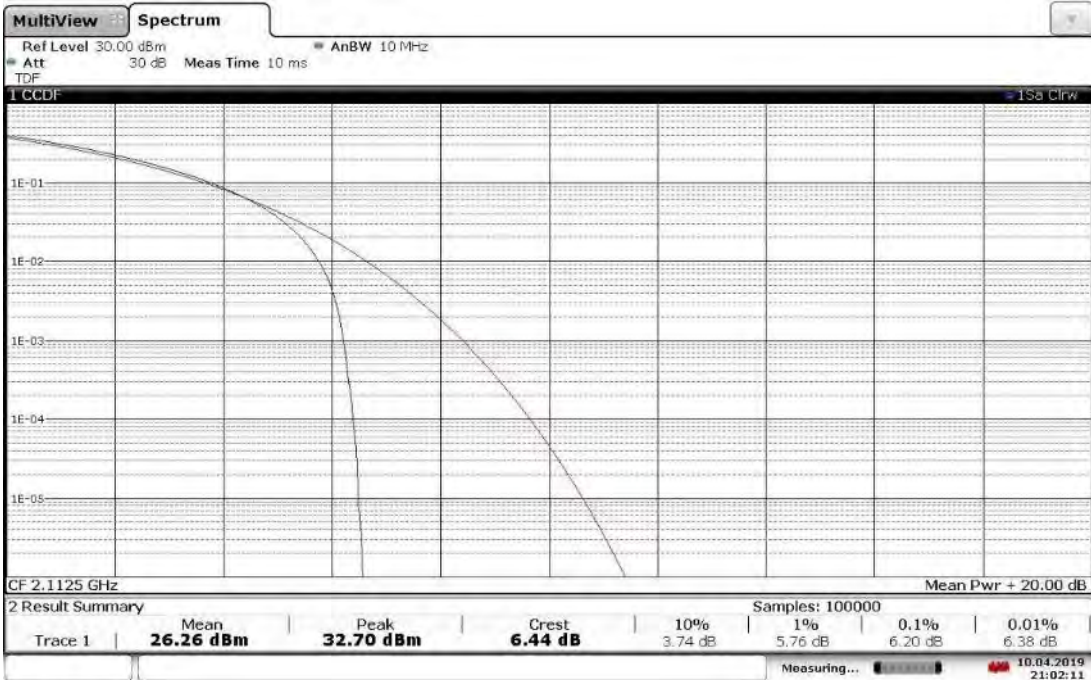
TM1.1-QPSK_5 MHz Bandwidth Slot 1 (Band 4), ANT1, Low Channel 2112.5 MHz, PAPR = 6.44 dB
