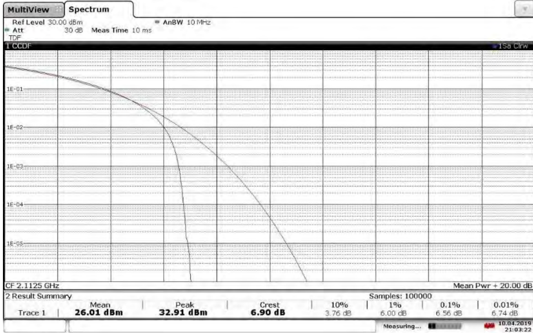
TM1.1-QPSK_5 MHz Bandwidth Slot 1 (Band 4), ANT0, Low Channel 2112.5 MHz, PAPR = 6.90 dB
