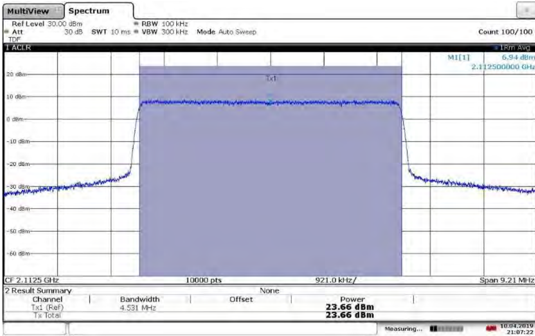
TM1.1-QPSK_5 MHz Bandwidth Slot 1 (Band 66), ANT0, Low Channel 2112.5 MHz, Output Power = 23.66 dBm
