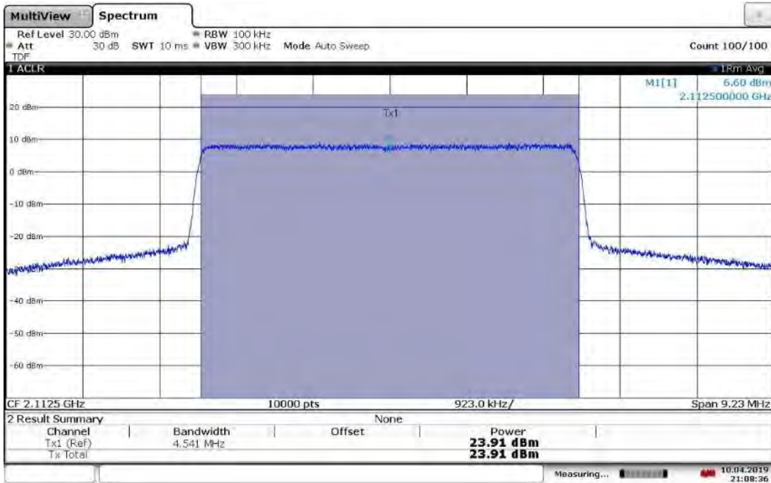
TM1.1-QPSK_5 MHz Bandwidth Slot 1 (Band 66), ANT1, Low Channel 2112.5 MHz, Output Power = 23.91 dBm
