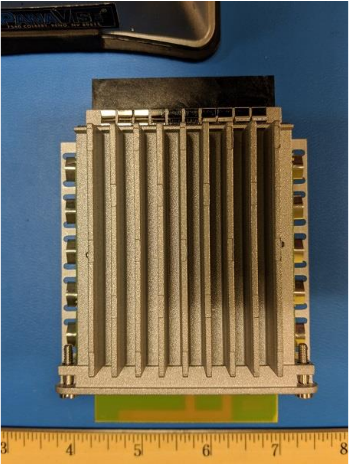
RM-Band66-Rear
