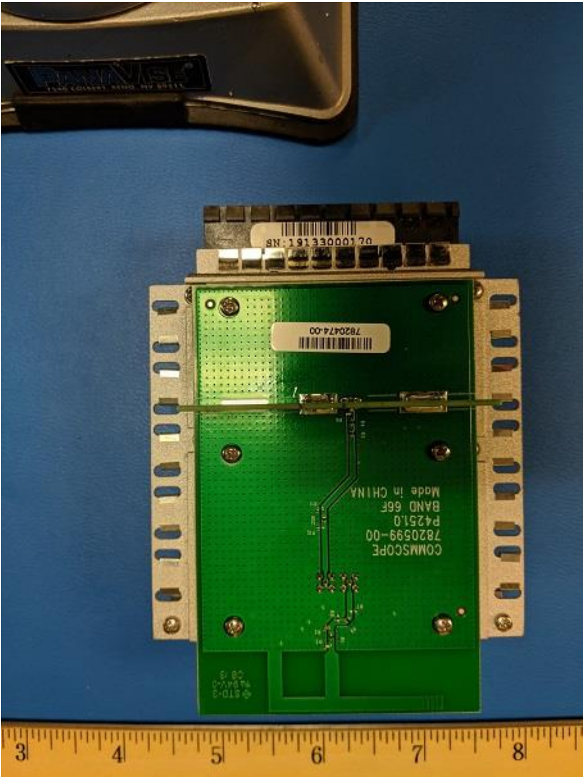
RM-Band66-Front
