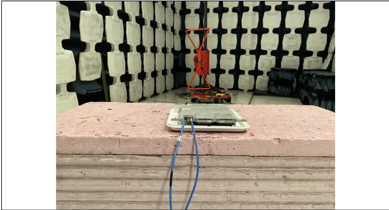
Radiated Emission Test below 1GHz Front View
