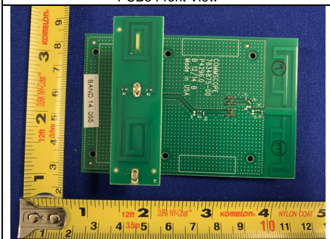
Antenna Front View
