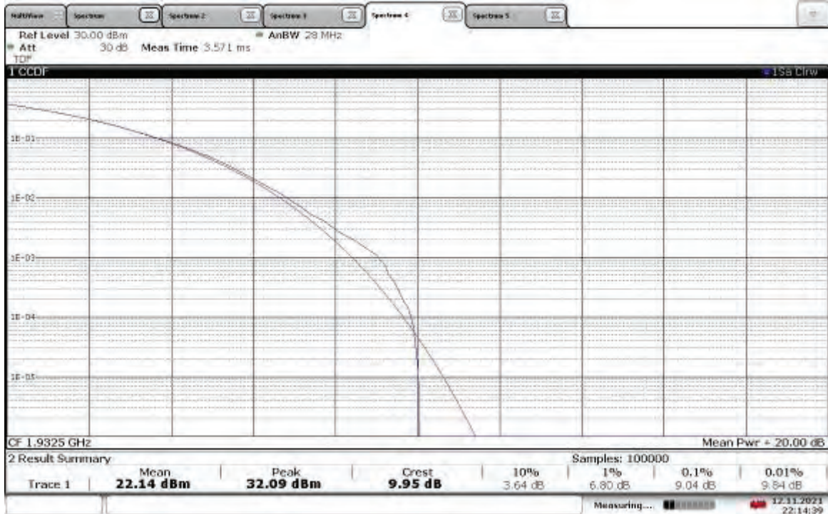
TM1.1-QPSK_5 MHz Bandwidth Slot 0 (Band 2), ANT1, Low Channel 1932.5 MHz, PAPR = 9.95 dB
