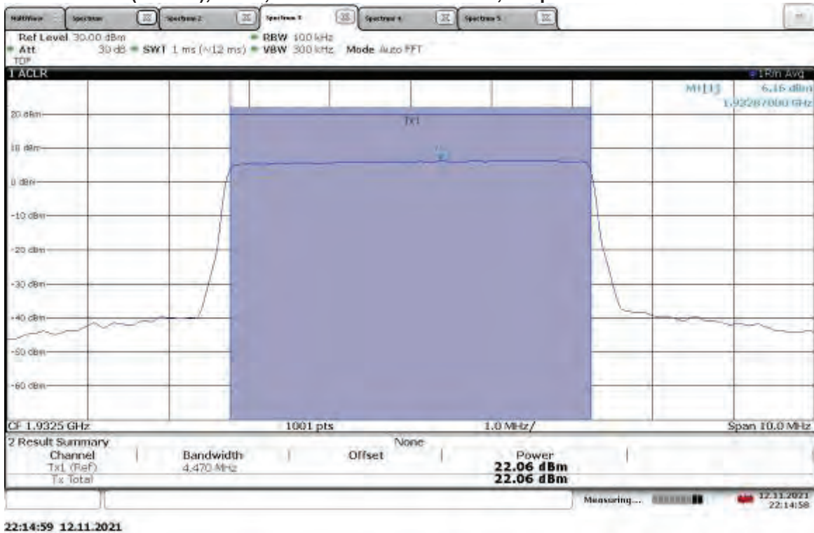
TM1.1-QPSK_5 MHz Bandwidth Slot 0 (Band 2), ANT1, Low Channel 1932.5 MHz, Output Power = 22.06 dBm
