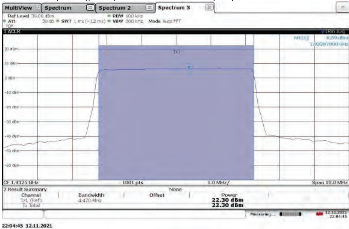
TM1.1-QPSK_5 MHz Bandwidth Slot 0 (Band 2), ANT0, Low Channel 1932.5 MHz, Output Power = 22.30 dBm
