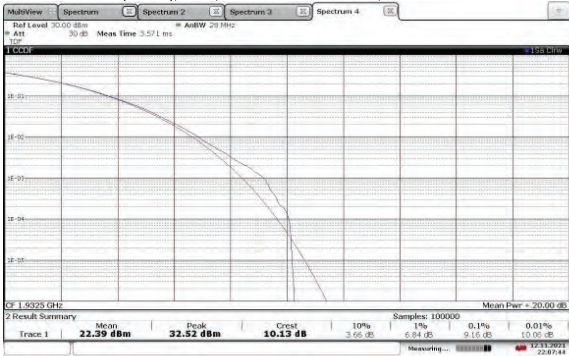
TM1.1-QPSK_5 MHz Bandwidth Slot 0 (Band 2), ANT0, Low Channel 1932.5 MHz, PAPR = 10.13 dB
