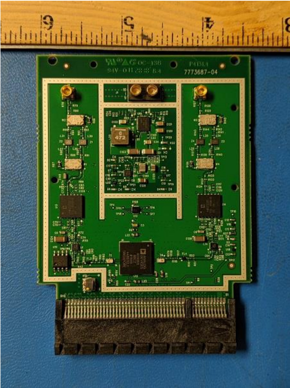
PCBA-Band2-Front
