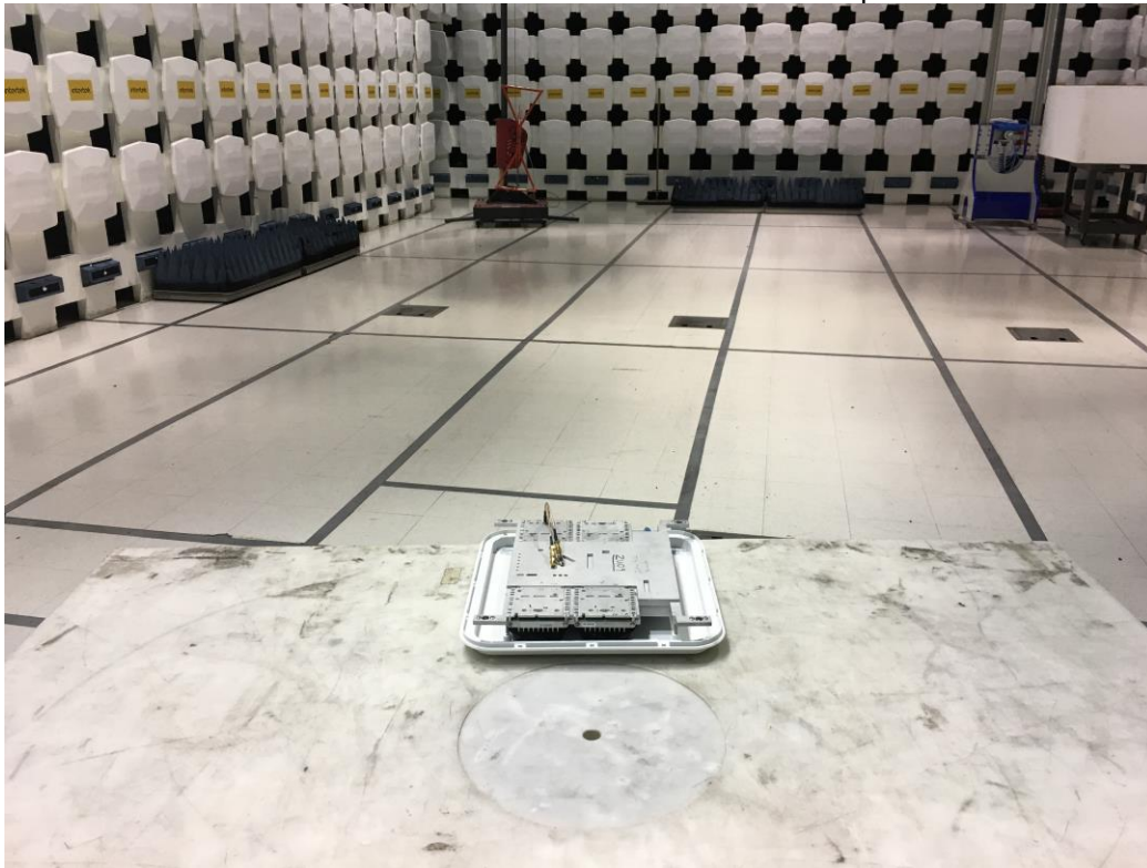
30-1000 MHz Radiated Emissions Test Setup
