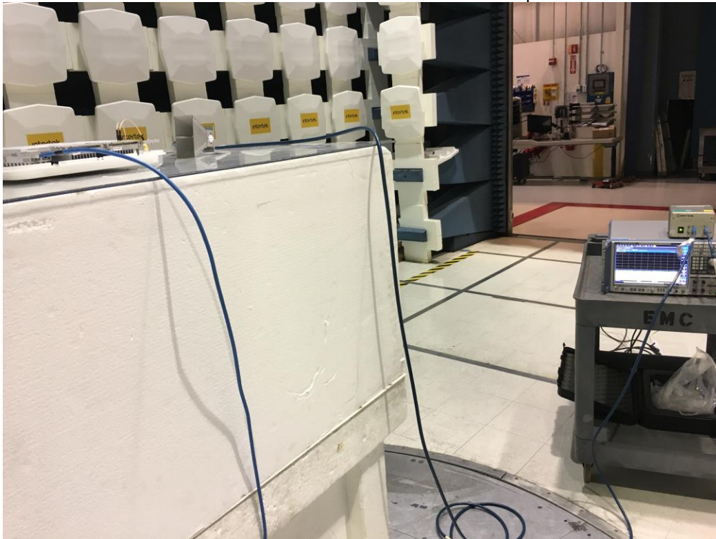
18-22 GHz Radiated Emissions Test Setup
