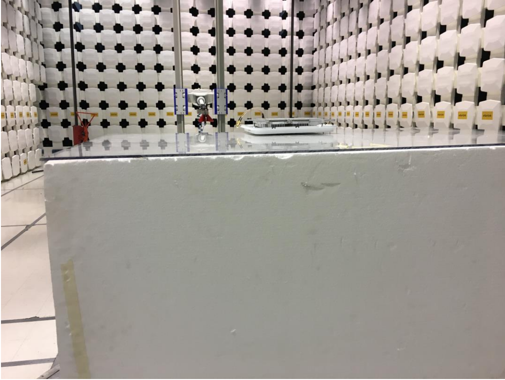
1-18 GHz Radiated Emissions Test Setup
