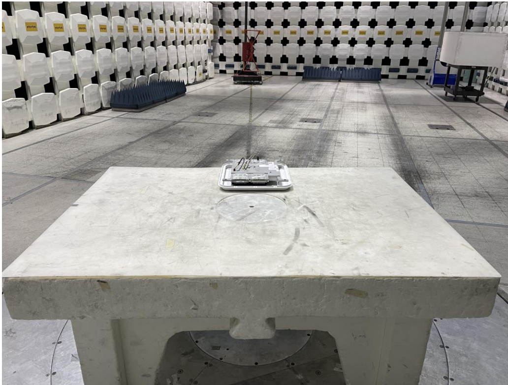
RPM-A5A11-B13 with W/ 4G LTE With OneCell® RP5200 – 30-1000 MHz Radiated Emissions
