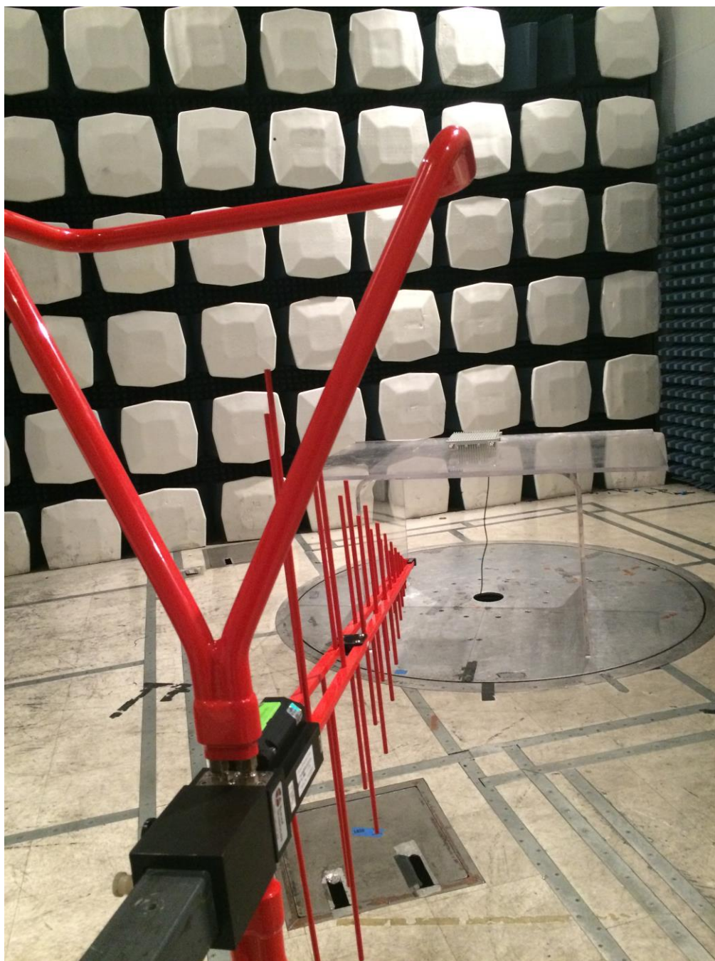
Photograph 1. Radiated Emissions, Below 1 GHz
