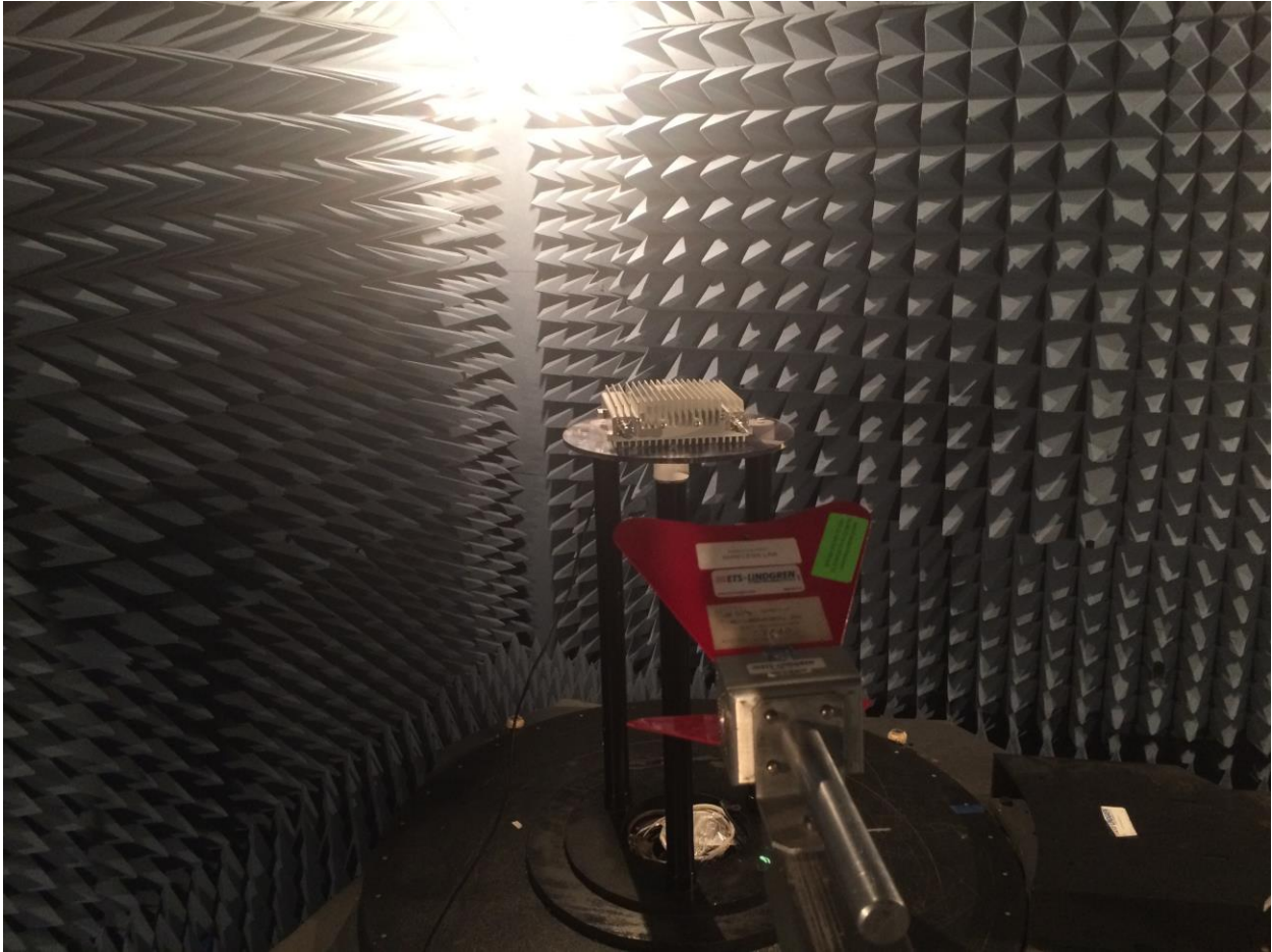
Photograph 2. Radiated Emissions, Above 1 GHz
