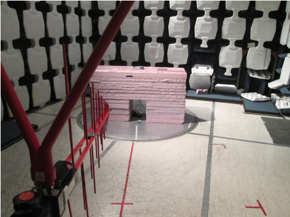
Radiated Emission - Rear 30MHz to 1GHz
