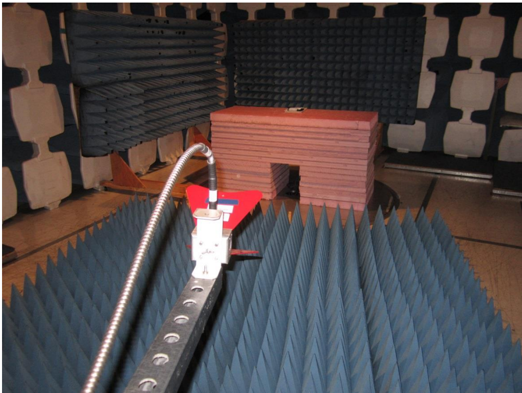
Radiated Emission - Front 1GHz to 6GHz
