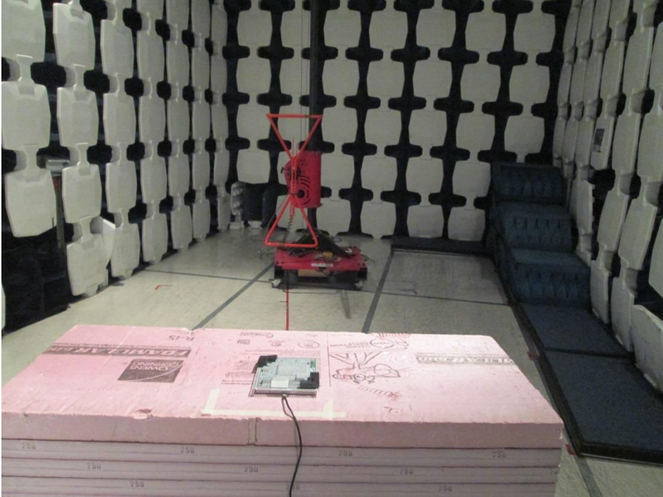
Radiated Emission - Rear 30MHz-1GHz
