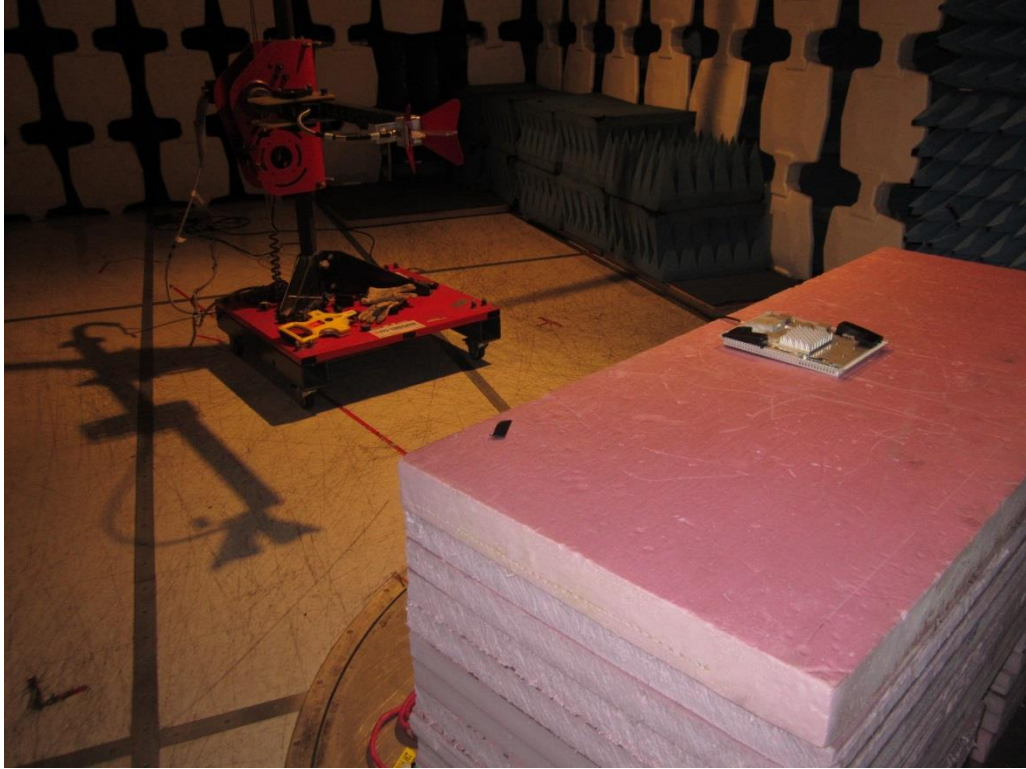
Radiated Emission - Rear 6GHz to 18GHz
