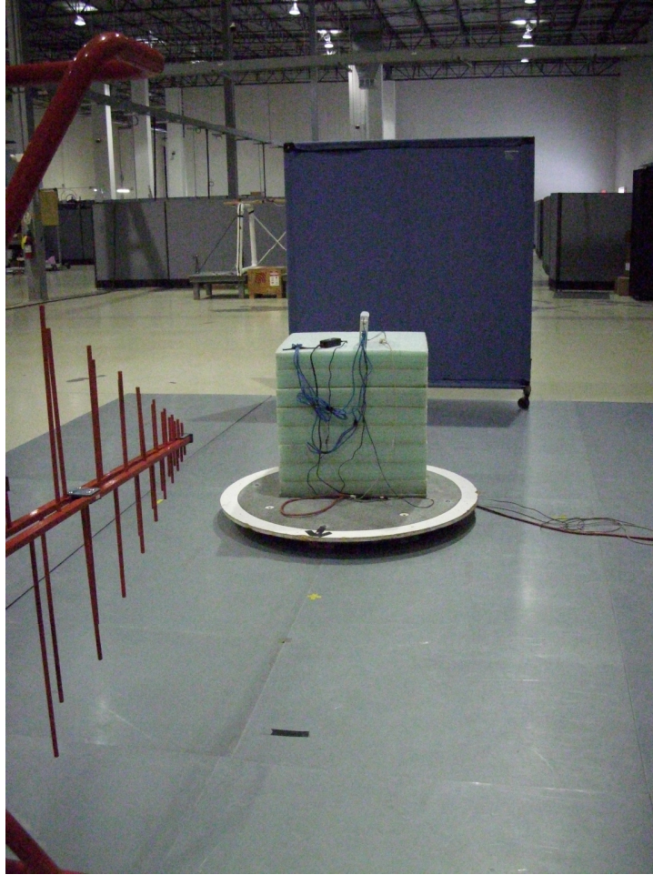
Radiated Emissions Measurements – OATS – Below 1GHz
