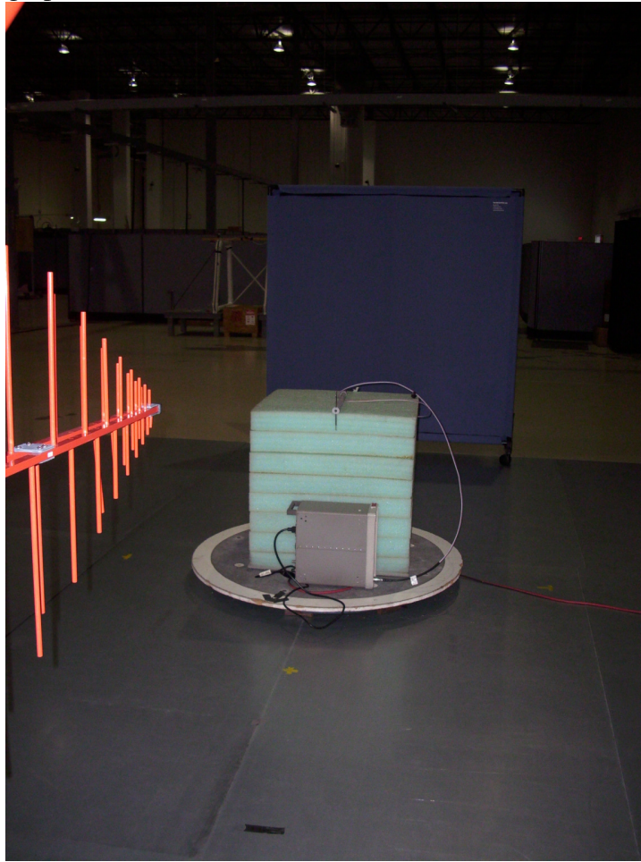
Substitution Method – OATS – Below 1GHz
