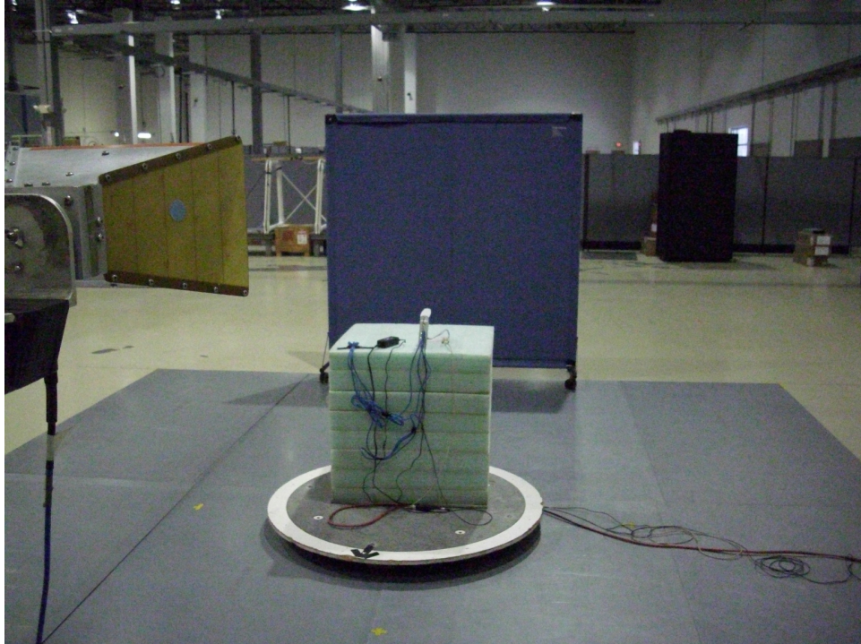
Radiated Emissions Measurements – OATS – Above 1GHz
