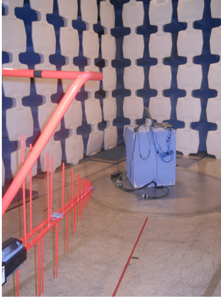
Radiated Emissions Measurements – Anechoic Chamber – Below 1GHz
