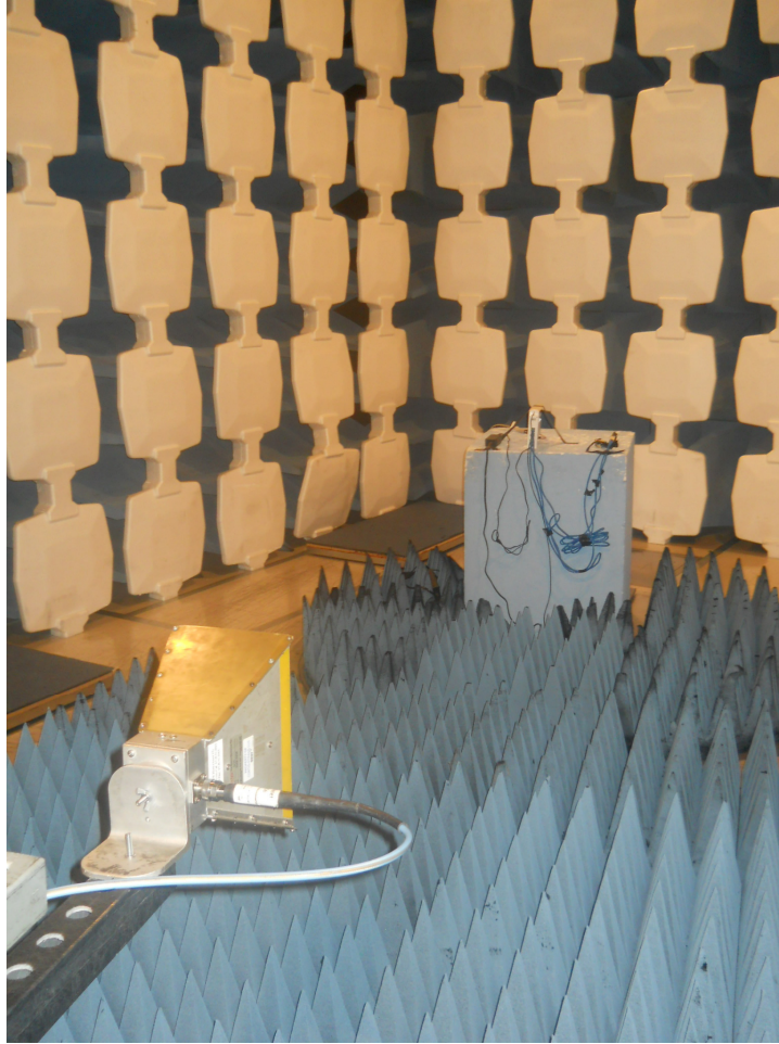
Radiated Emissions Measurements – Anechoic Chamber – Above 1GHz
