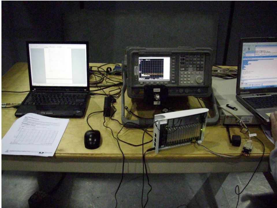
Conducted Measurements
