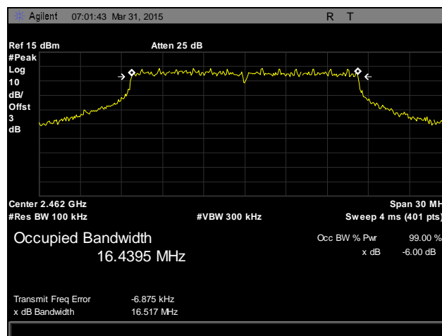
Plot 8. Occupied Bandwidth, 802.11g 20 MHz, High Channel, MIMO
