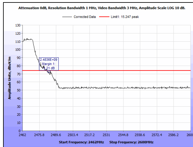
Plot 60. Radiated Band Edge, 802.11n 20 MHz, High Channel, 2462 MHz @ 2483.5 MHz, Peak
