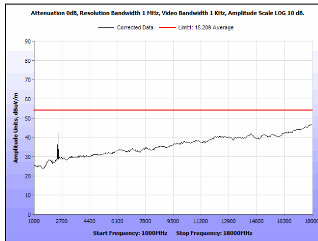
Plot 47. Radiated Spurious Emissions, 802.11n 40 MHz, High Channel, 2452 MHz, 1 GHz – 18 GHz, Average
