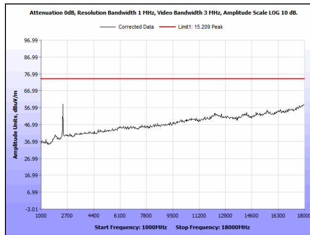
Plot 29. Radiated Spurious Emissions, 802.11g 20 MHz, Low Channel, 2412 MHz, 1 GHz – 18 GHz, Peak
