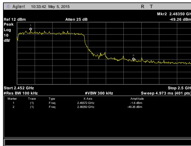
Plot 104. Conducted Band Edge, 802.11n 40 MHz, High Channel, Port 2
