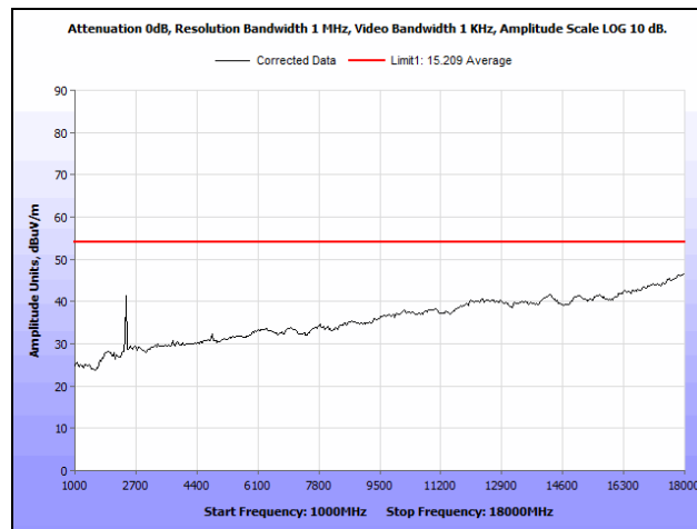
Plot 35. Radiated Spurious Emissions, 802.11n 20 MHz, Low Channel, 2412 MHz, 1 GHz – 18 GHz, Average
