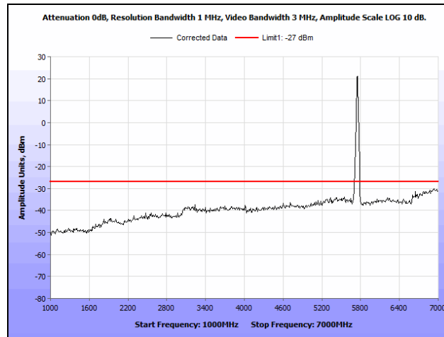
Plot 24. Radiated Spurious Emissions, 5745 MHz, 802.11ac 20 MHz, 1 GHz – 7 GHz
