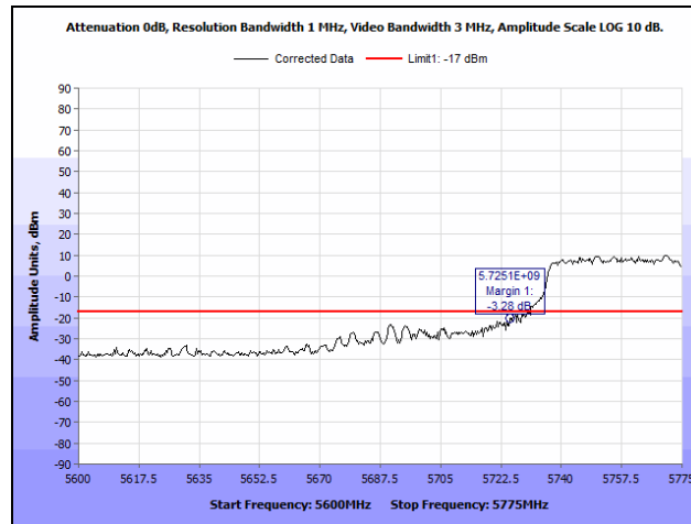
Plot 61. Radiated Band Edge, 802.11ac 80 MHz, 5775 MHz @ 5725 MHz
