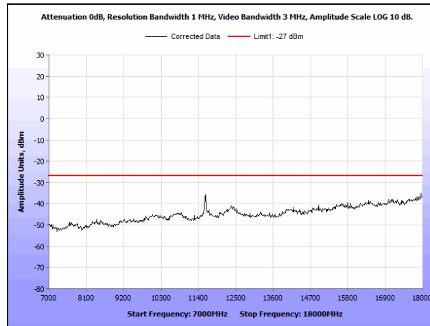
Plot 42. Radiated Spurious Emissions, 5795 MHz, 802.11ac 40 MHz, 7 GHz – 18 GHz
