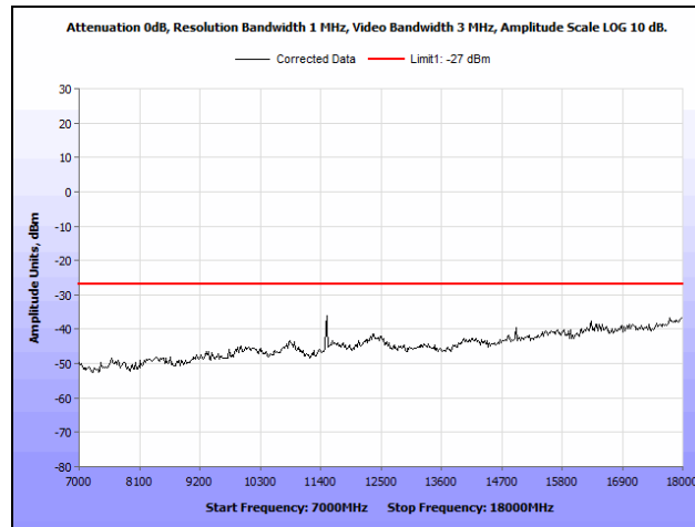
Plot 39. Radiated Spurious Emissions, 5755 MHz, 802.11ac 40 MHz, 7 GHz – 18 GHz
