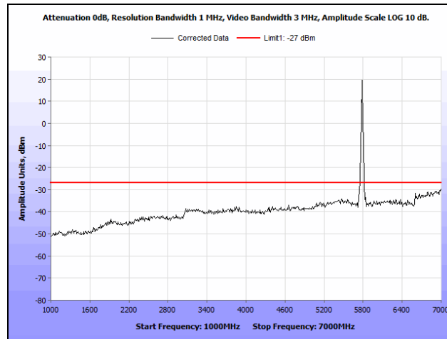
Plot 27. Radiated Spurious Emissions, 5785 MHz, 802.11ac 20 MHz, 1 GHz – 7 GHz
