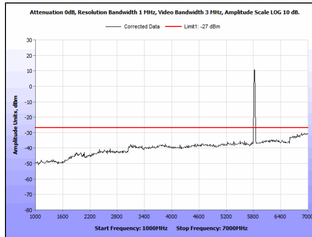
Plot 36. Radiated Spurious Emissions, 5825 MHz, 802.11n 20 MHz, 1 GHz – 7 GHz
