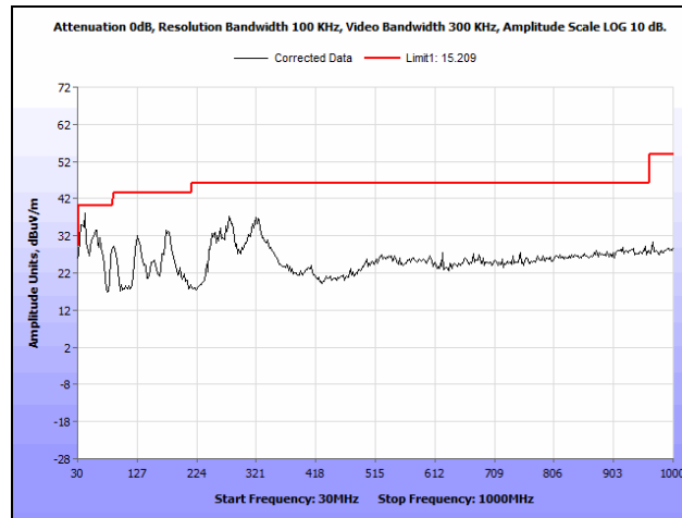
Plot 48. Radiated Spurious Emissions, 5775 MHz, 802.11ac 80 MHz, 30 MHz – 1 GHz
